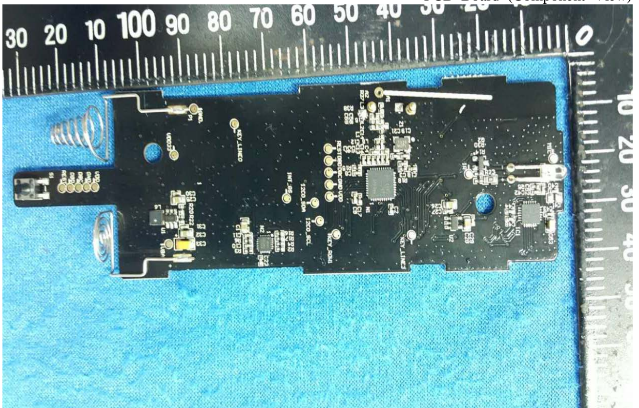
Figure 6 PCB Board (Component View)
