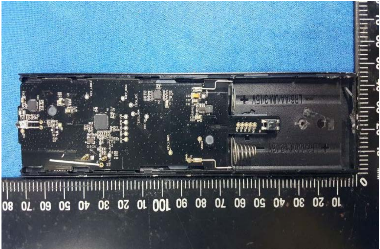
Figure 3 Internal View
