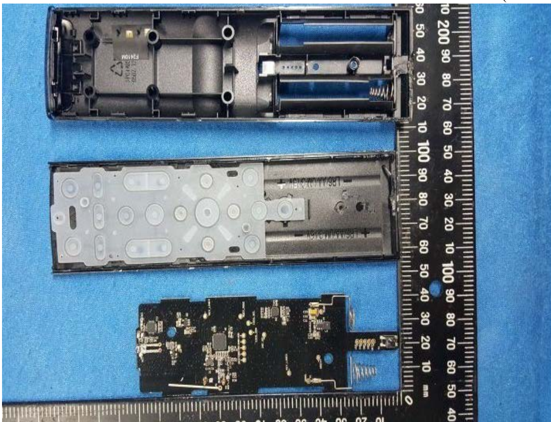
Figure 2 Internal View(Cover Removed)
