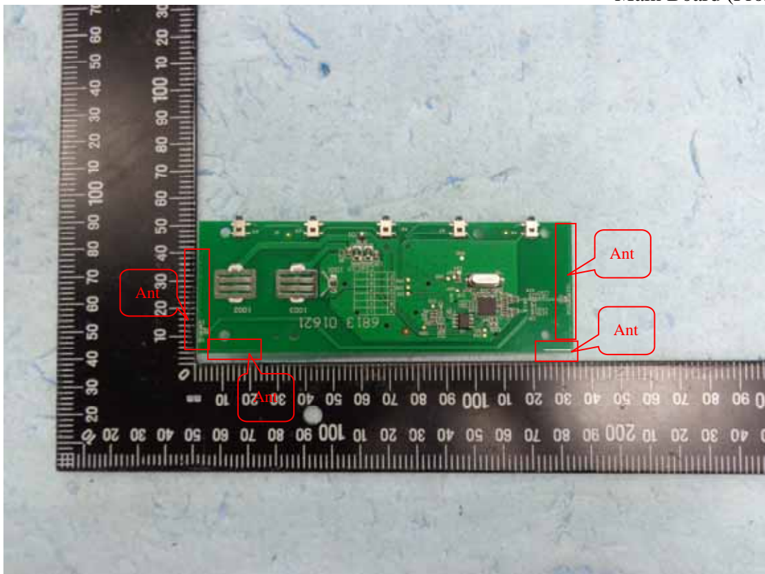
Figure 6 Main Board (Front View)
