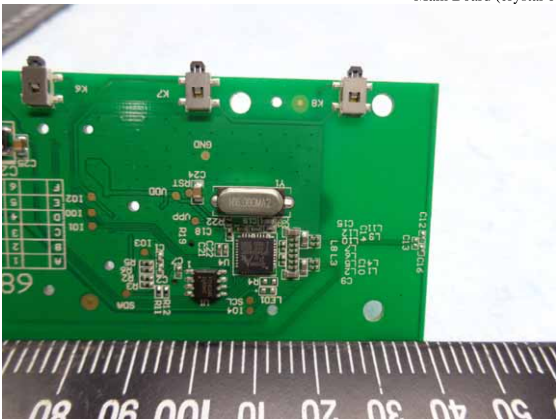
Figure 8 Main Board (crystal oscillator)
