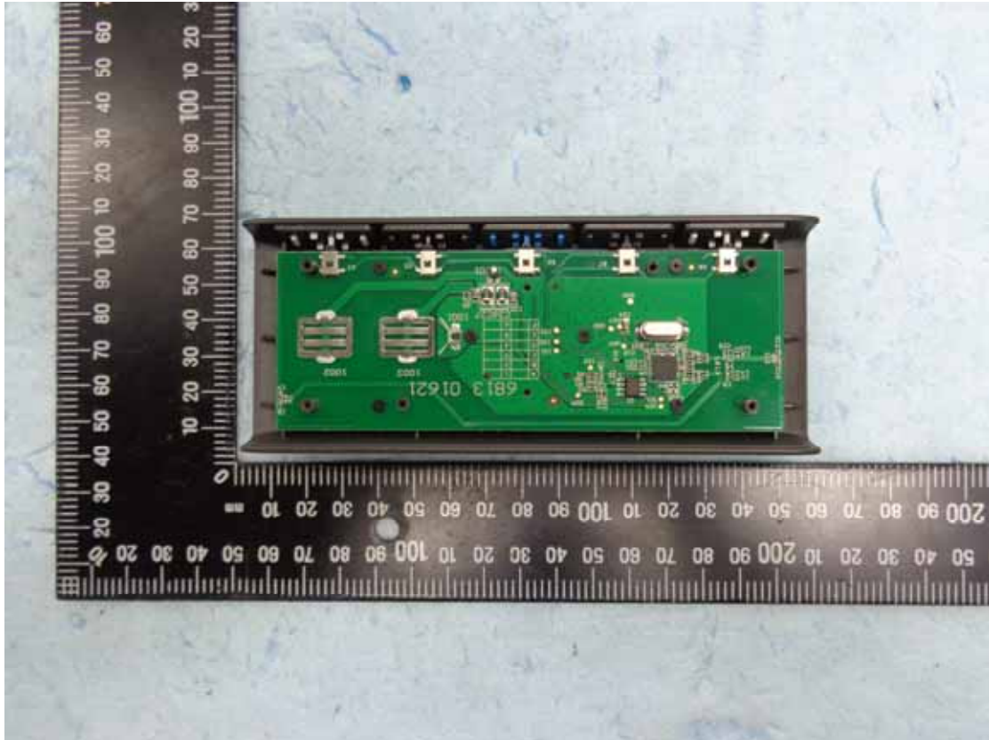
Figure 3 Internal View
