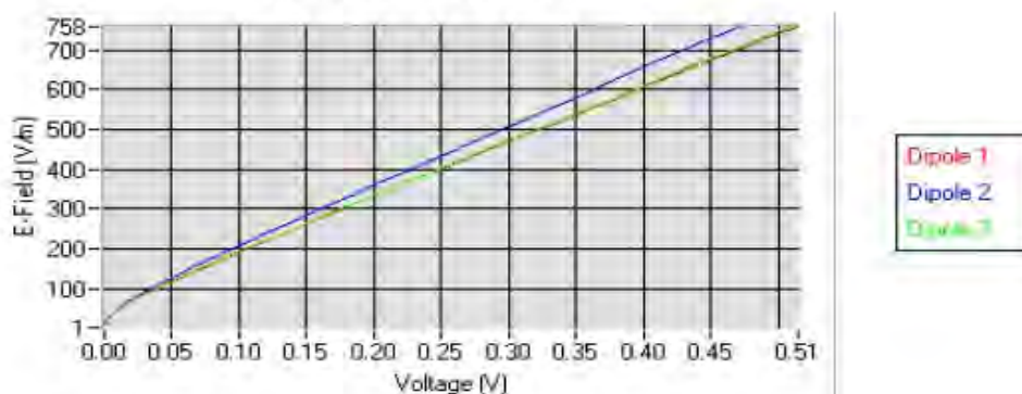
Calibration curves
