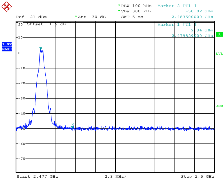
(Plot 4.5.2.1 B: Hopping Mode @ GFSK)
