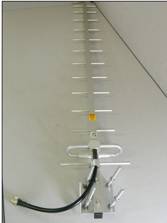
Figure 13: External Photo – Yagi Antenna
