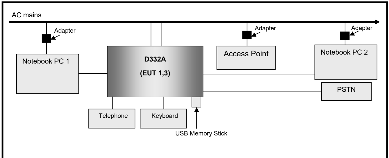
[Conducted Emission for EUT #1, and EUT #3]
