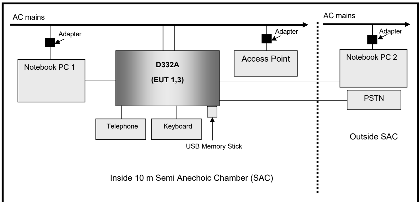
[Radiated Emission for EUT #1, and EUT #3]
