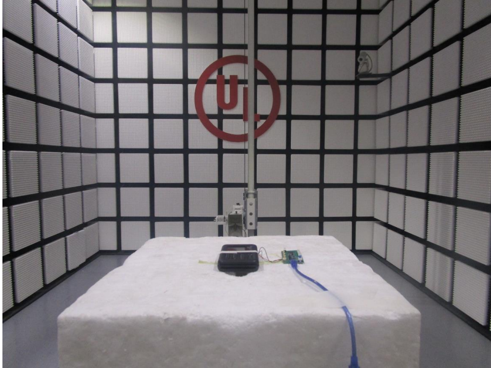
RADIATED RF MEASUREMENT SETUP (Above 1G – Y axis) (BT/BLE)
