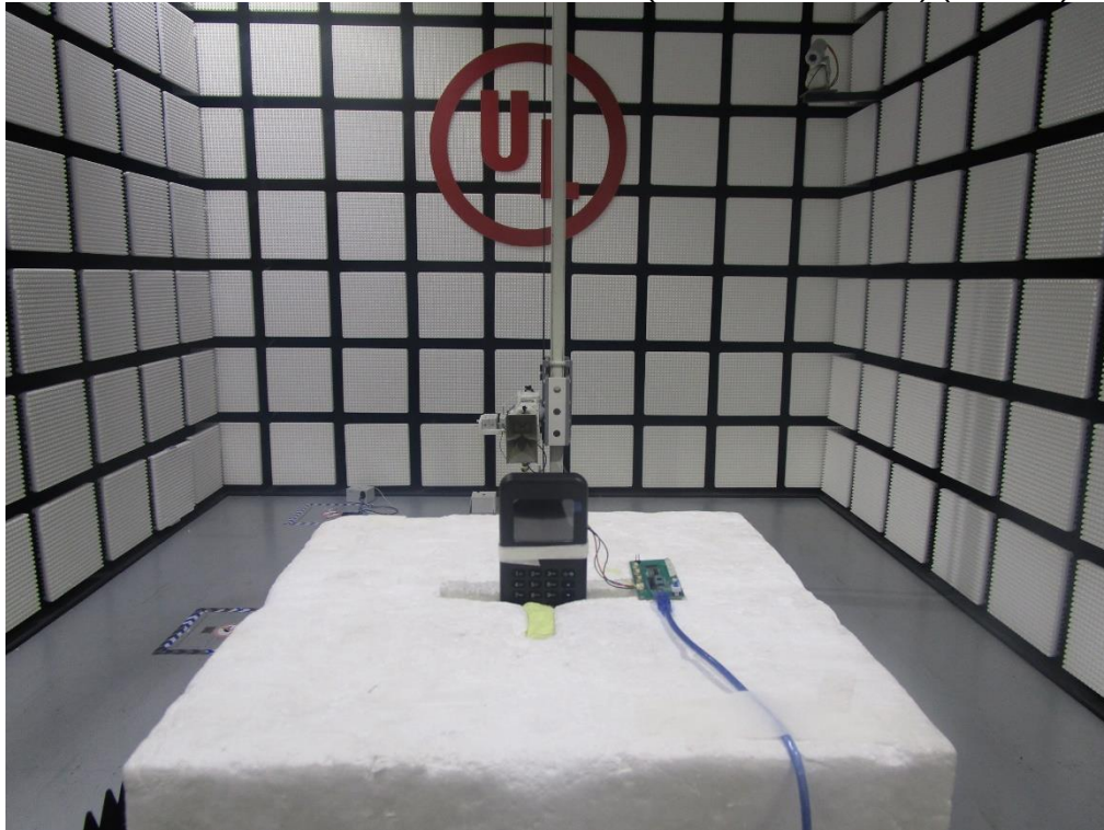
RADIATED RF MEASUREMENT SETUP (Above 1G – Z axis) (BT/BLE)
