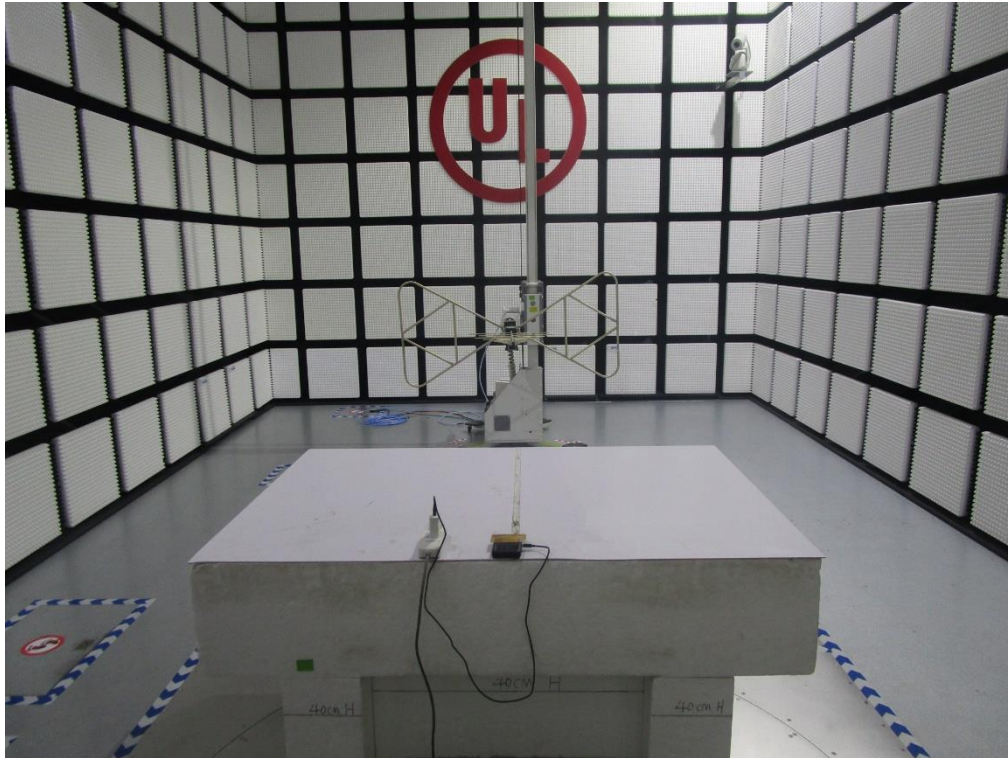
Radiated Disturbance Below 1 GHz and Above 30 MHz (BT/BLE)
