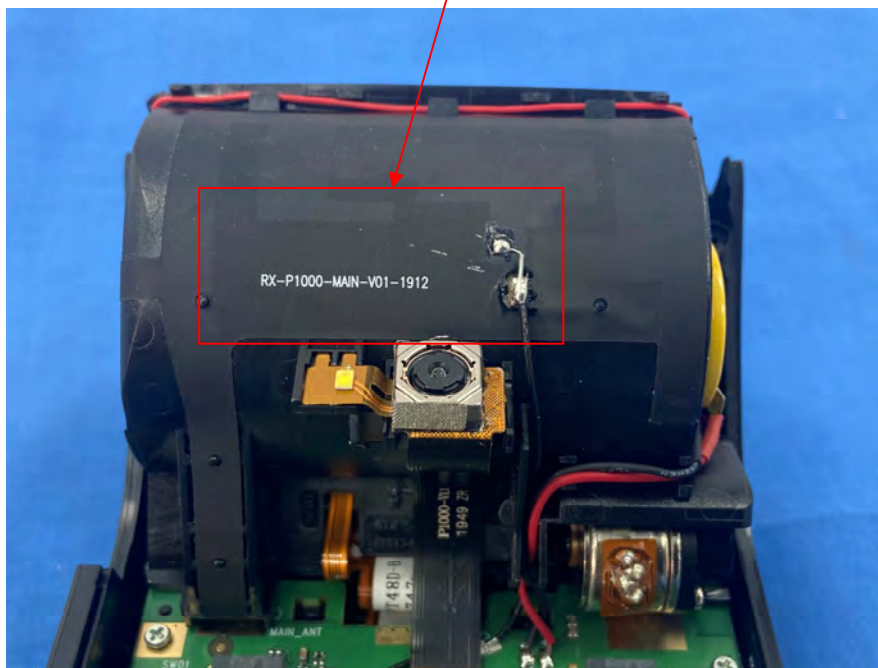
LTE Diversity Antenna
