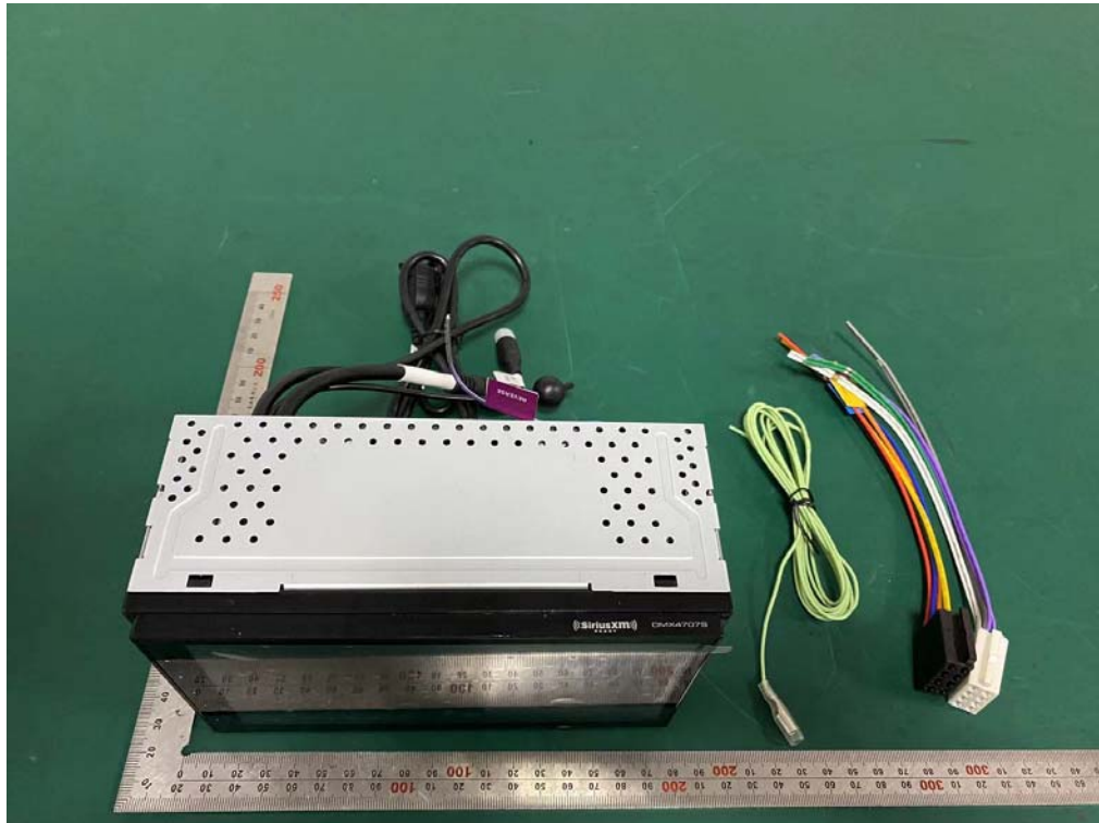
External Photos M/N: DMX4707S
