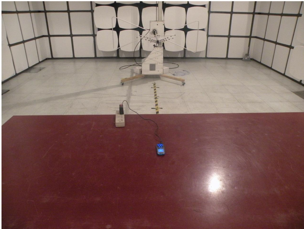
Part 15.247 Blow 1GHz
