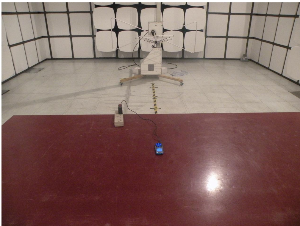
Part 22 and Part 24 Blow 1GHz
