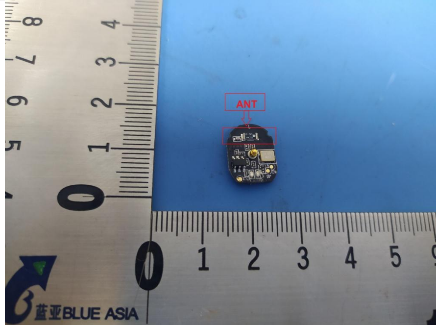
Antenna Requirement
