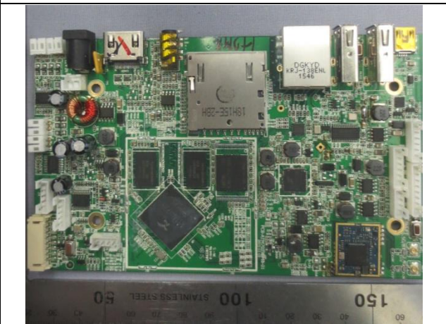
Radiator removed
