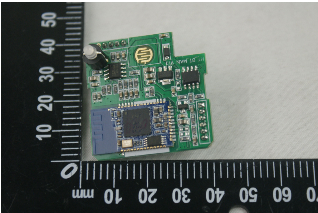
THE MIAN BOARD 2 (Front)
