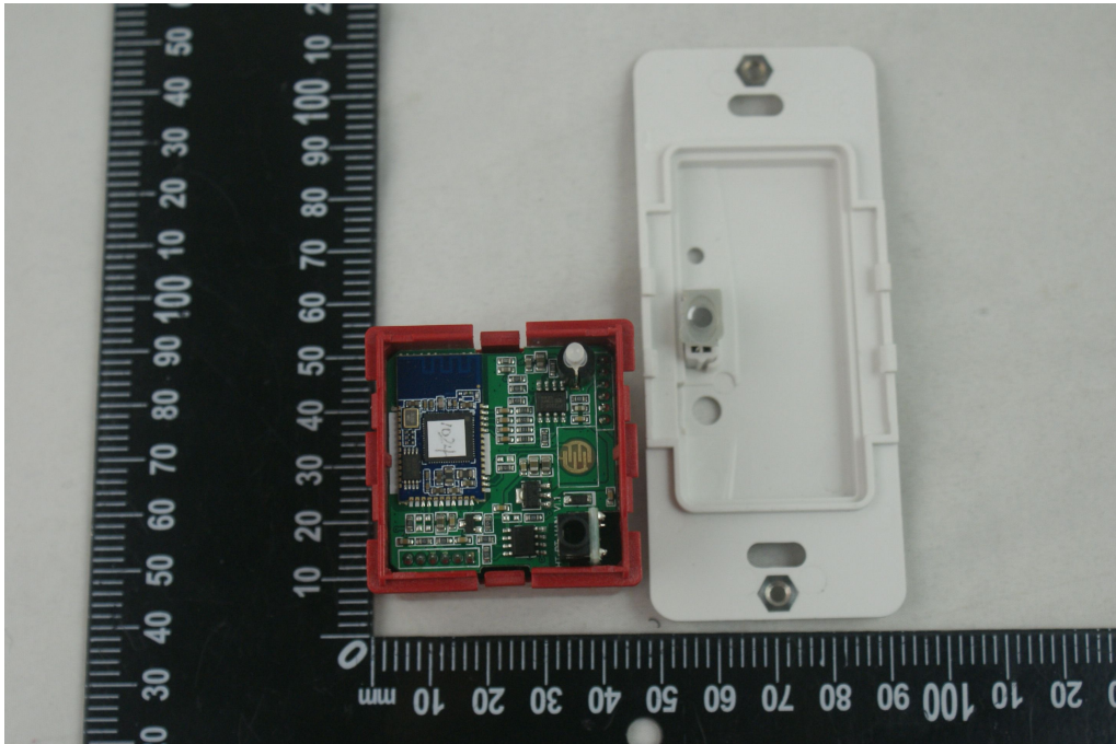
THE UNCOVER EUT VIEW 1
