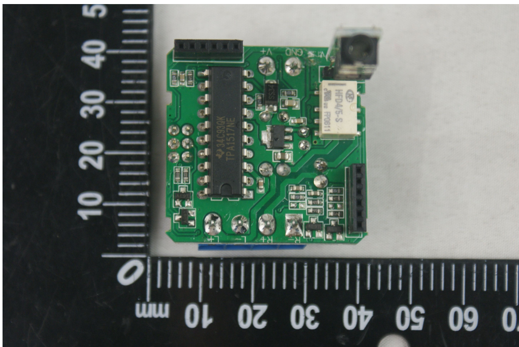
THE MIAN BOARD 1 (Front)
