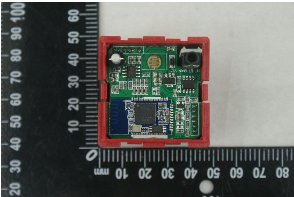
THE UNCOVER EUT VIEW 2
