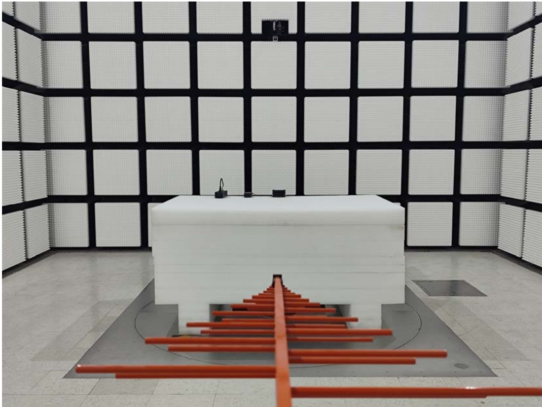
Radiated Emission Below 1GHz Rear View-M1
