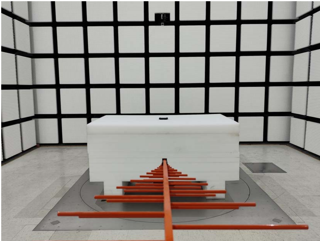
Radiated Emission Below 1GHz View-M3
