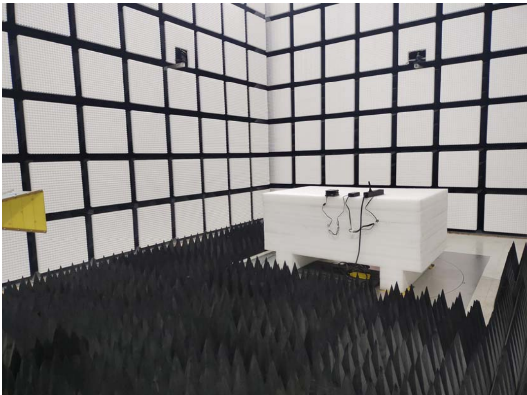
Radiated Emission Above 1GHz Rear View-M1
