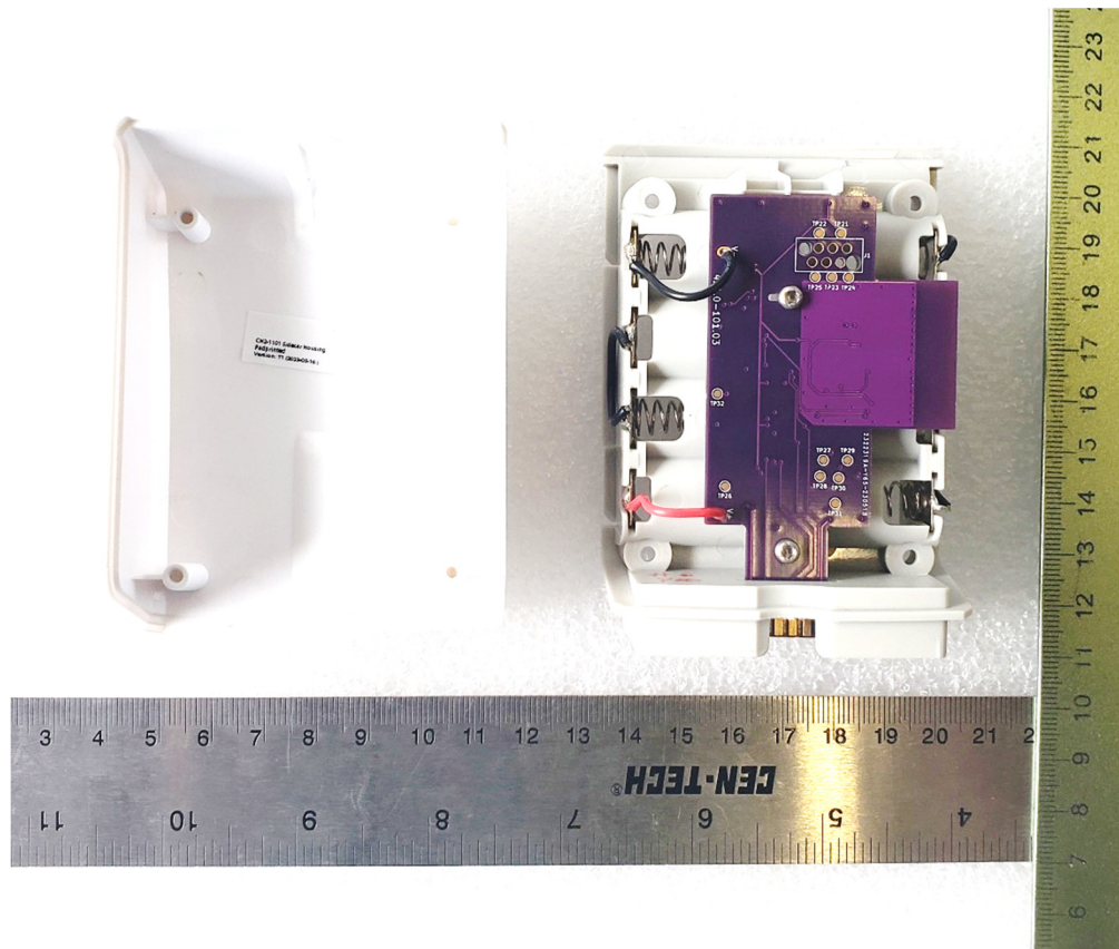
Figure 1. EUT, Front Cover Removed
