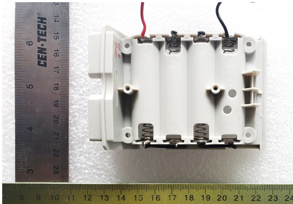
Figure 4. Enclosure with Main PCB Removed
