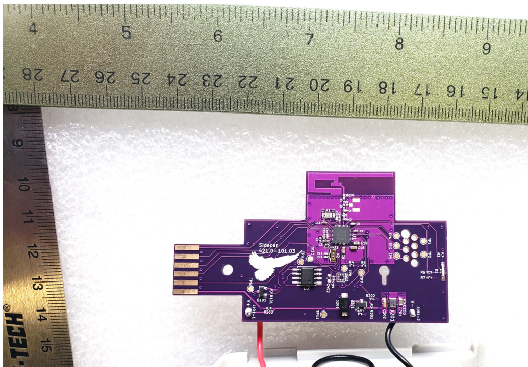
Figure 3. Front of Main PCB
