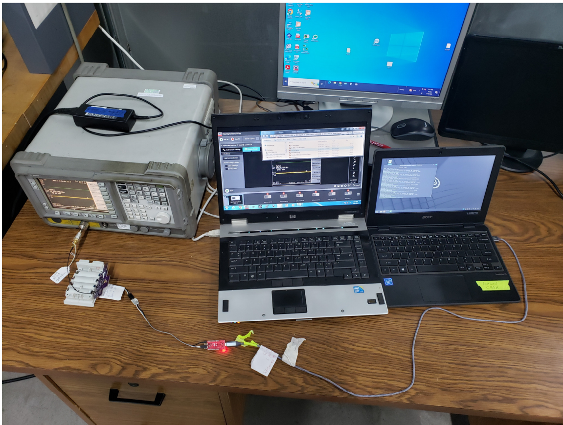
Figure 6. Bench Test Setup
