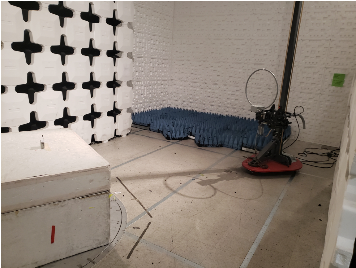
Figure 2. Radiated Emissions Test Setup, .15 MHz to 300 MHz
