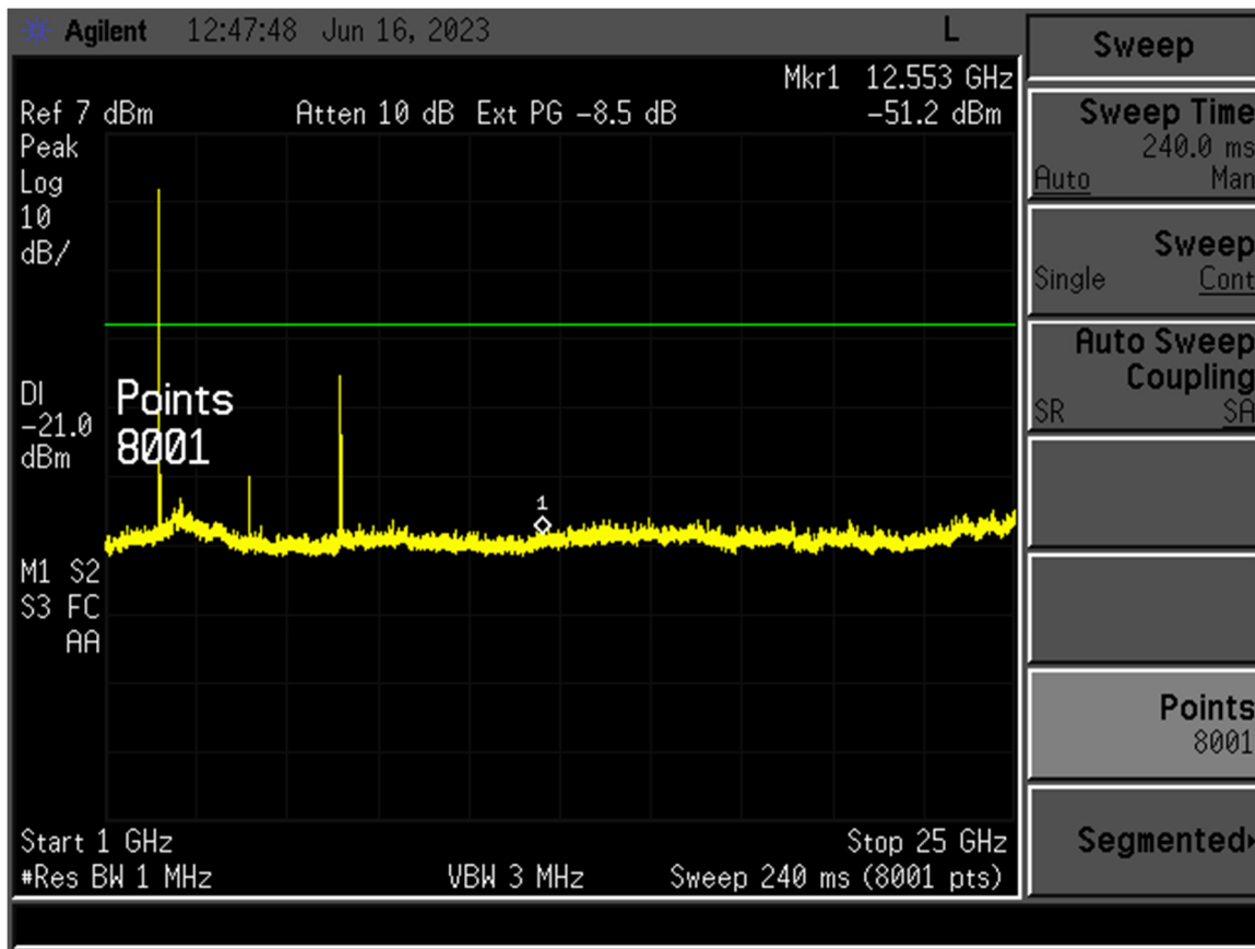
Figure 3. Channel 0, 1 – 25 GHz
