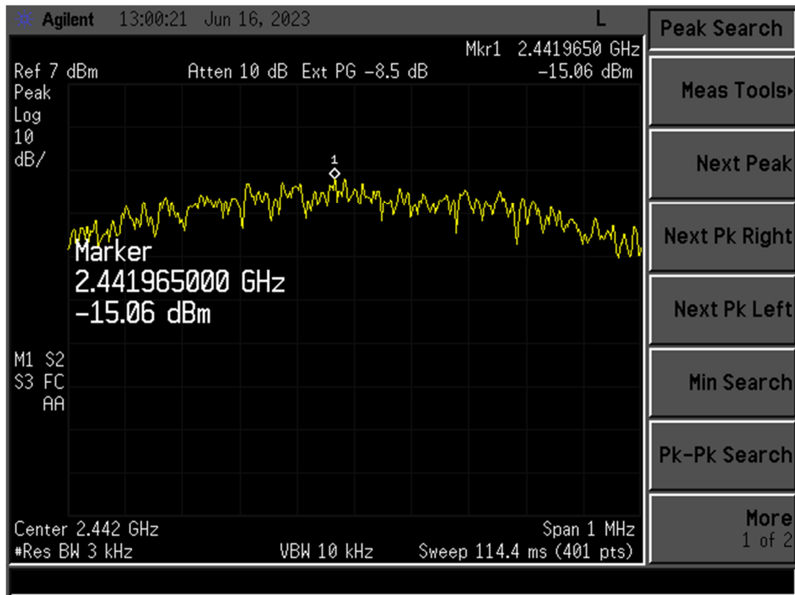
Figure 20. Power Spectral Density, Mid Channel
