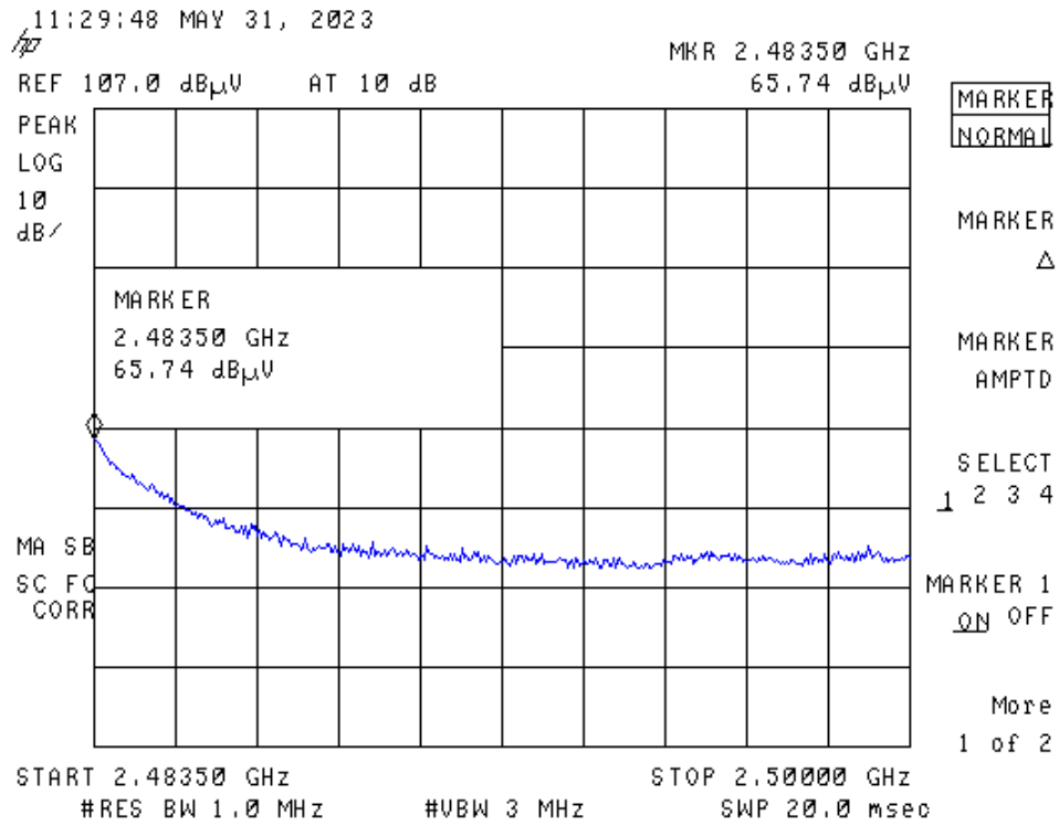
Figure 11. High Channel Restricted Band – Peak
