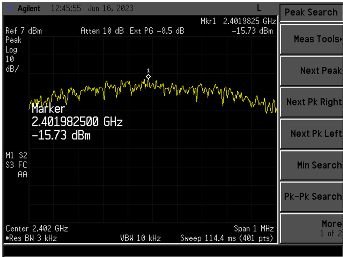
Figure 19. Power Spectral Density, Low Channel
