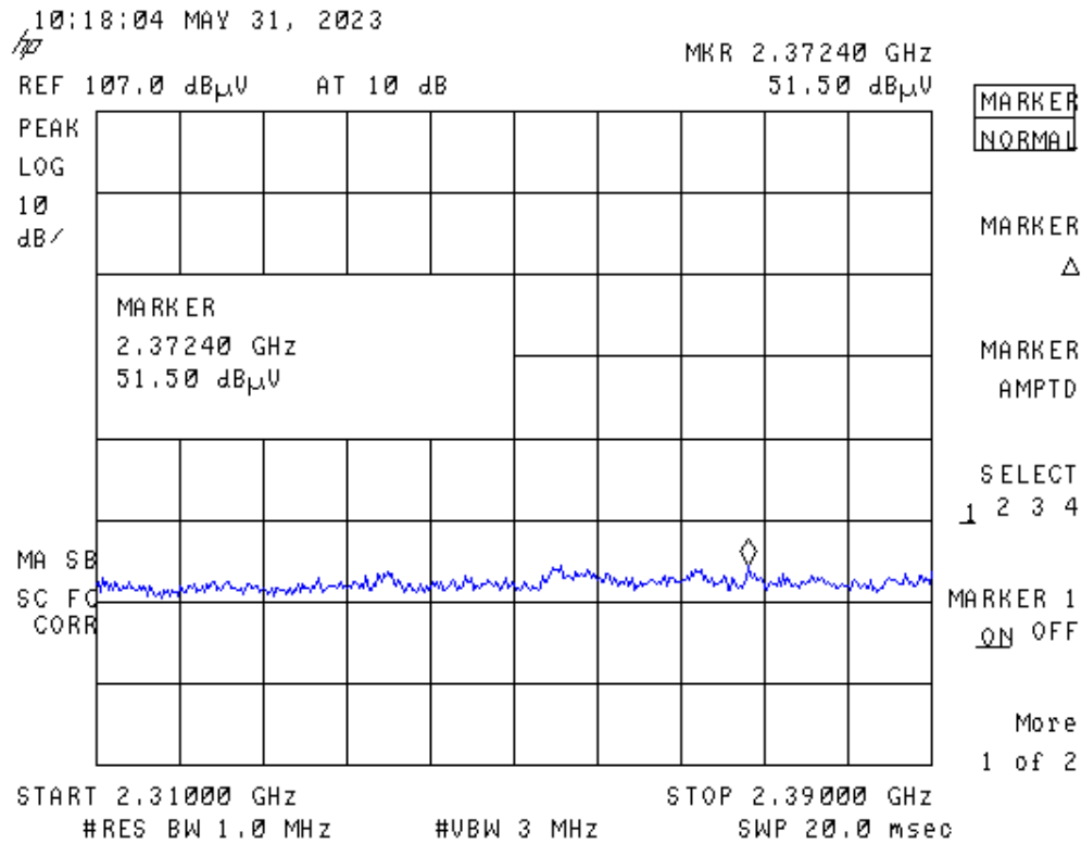
Figure 9. Low Channel Restricted Band - Peak
