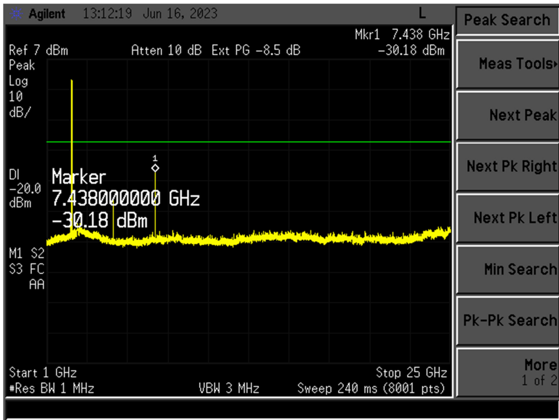
Figure 7. Channel 39, 1 - 25 GHz
