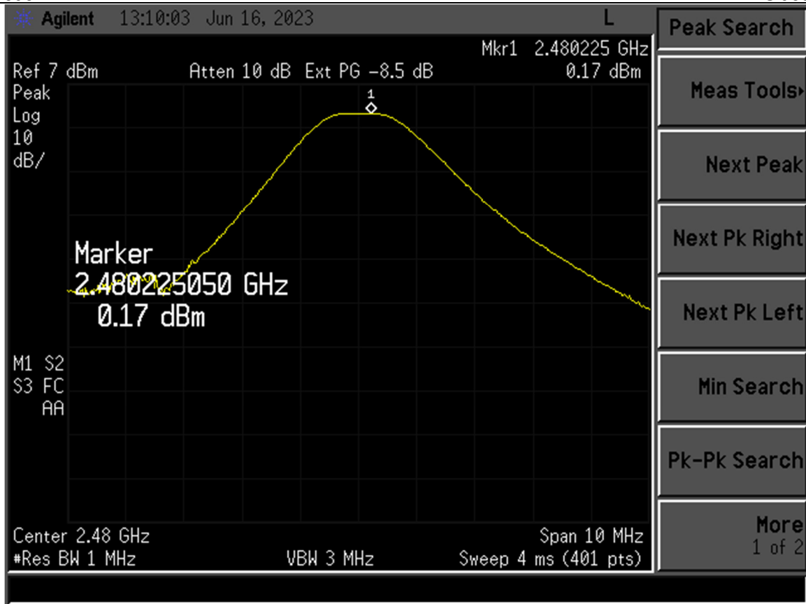
Figure 18. Peak Antenna Conducted Output Power, High Channel
