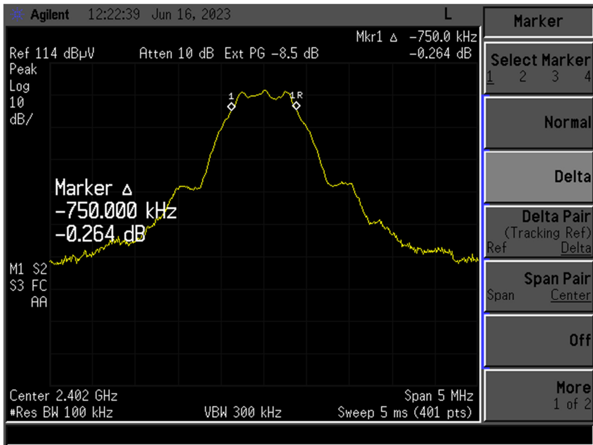
Figure 13. 6 dB Bandwidth Low Channel
