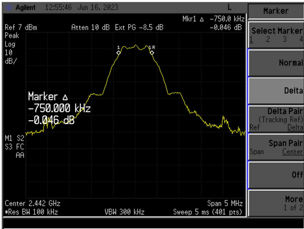
Figure 14. 6 dB Bandwidth Mid Channel
