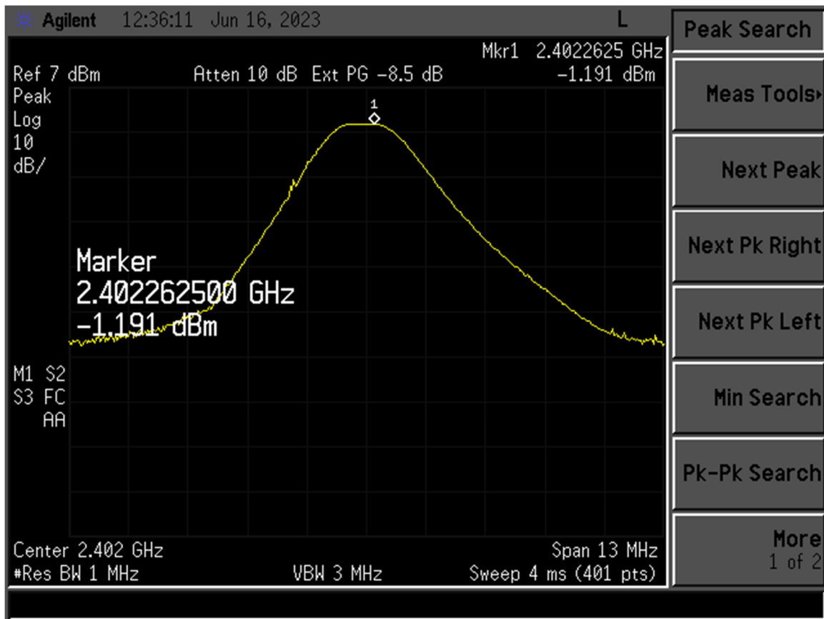
Figure 16. Peak Antenna Conducted Output Power, Low Channel
