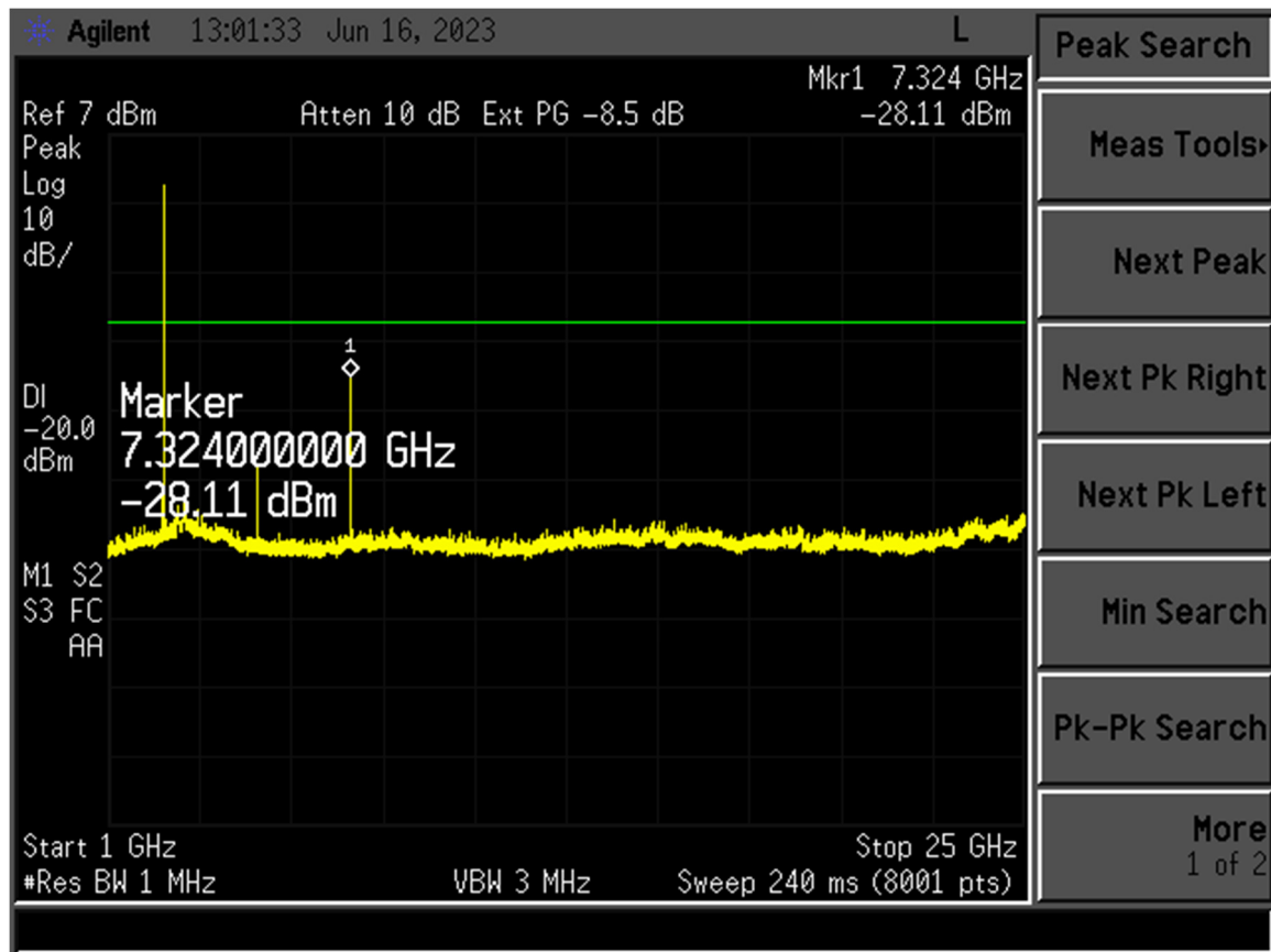
Figure 5. Channel 20, 1 – 25 GHz
