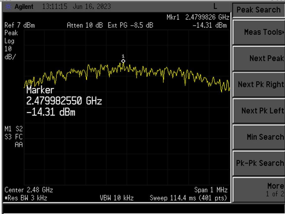
Figure 21. Power Spectral Density, High Channel
