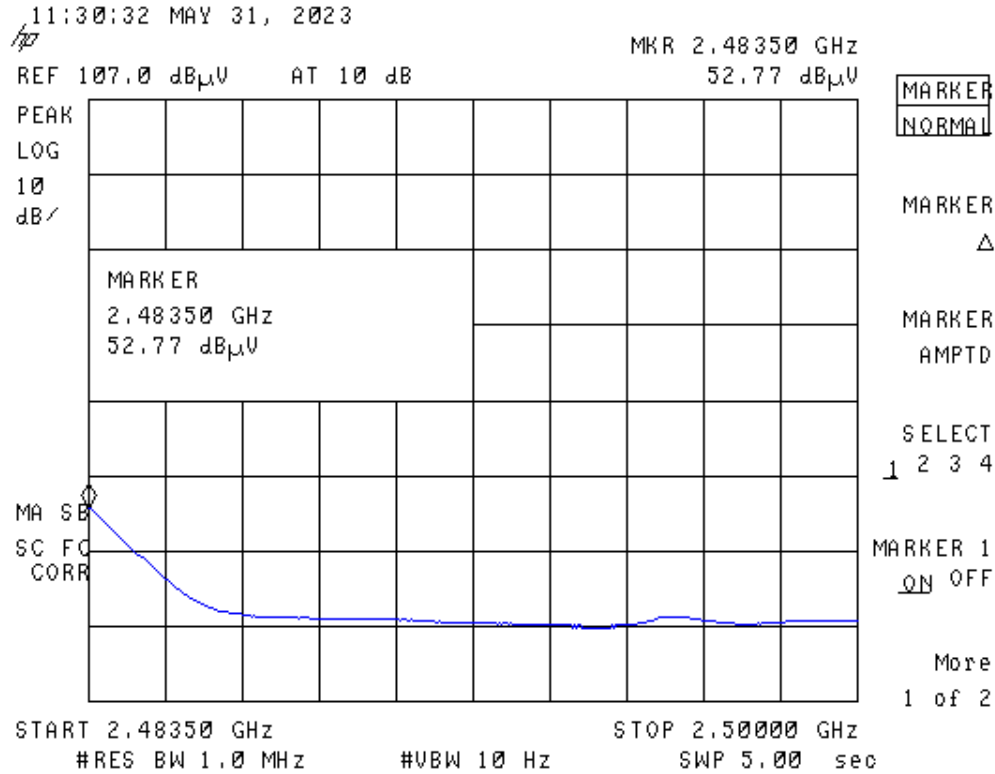
Figure 12. High Channel Restricted Band – Average
