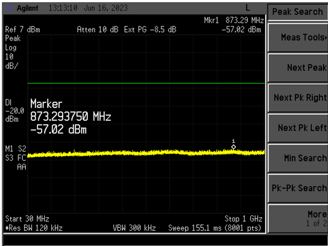
Figure 6. Channel 39, 30-1000 MHz
