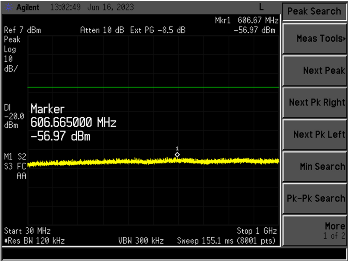
Figure 4. Channel 20, 30-1000 MHz
