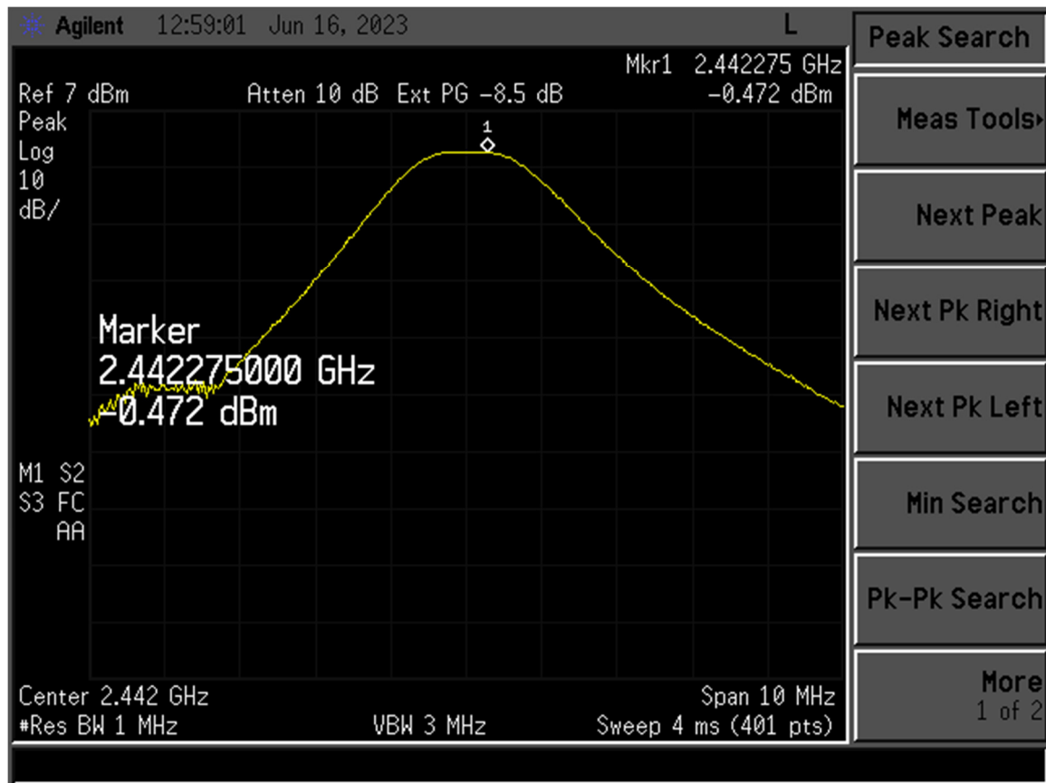
Figure 17. Peak Antenna Conducted Output Power, Mid Channel
