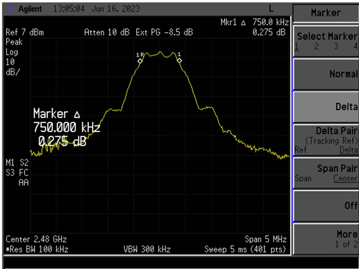
Figure 15. 6 dB Bandwidth High Channel
