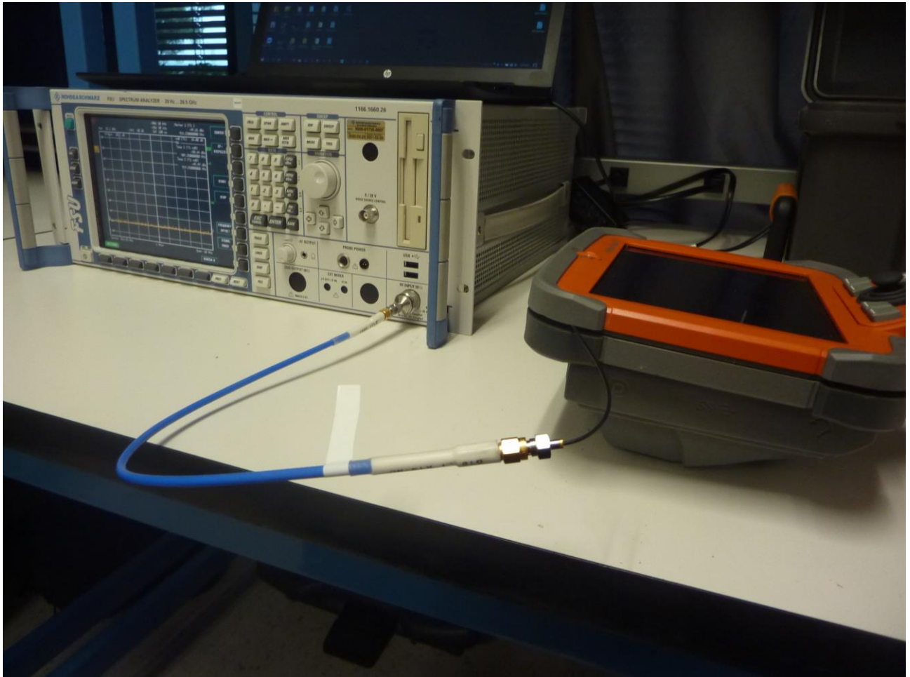
Figure 5: EUT Conducted Setup
