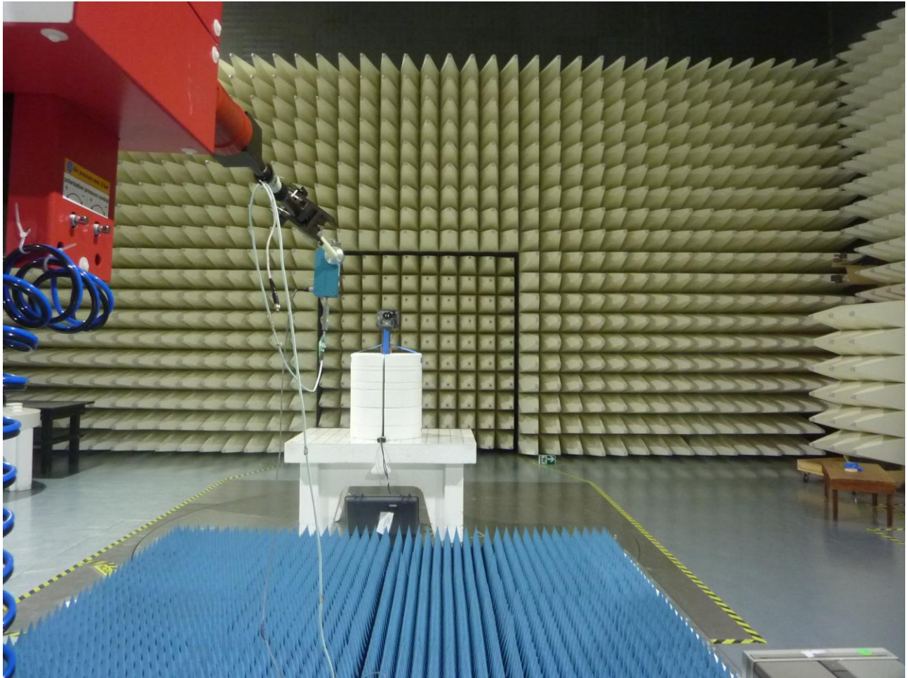
Figure 3: Test Setup for Radiated Emissions Above 18GHz
