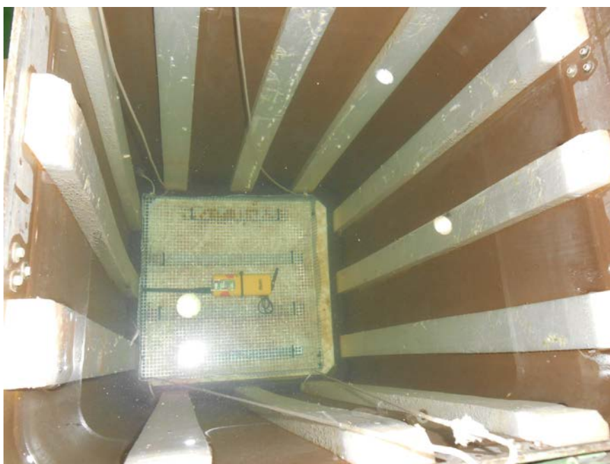
SPECIMEN TRA-021534-S2 SECURED TO A WEIGHTED FRAME FOR IPX7 IMMERSION
