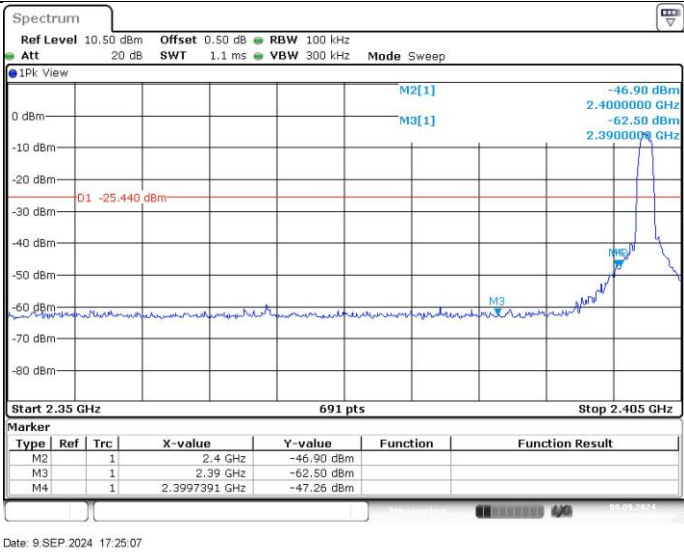
3DH5_Ant1_Low_2402
