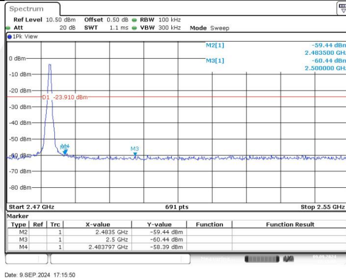
DH5_Ant1_High_2480
