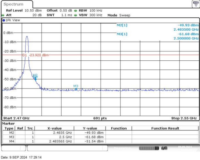
3DH5_Ant1_High_2480
