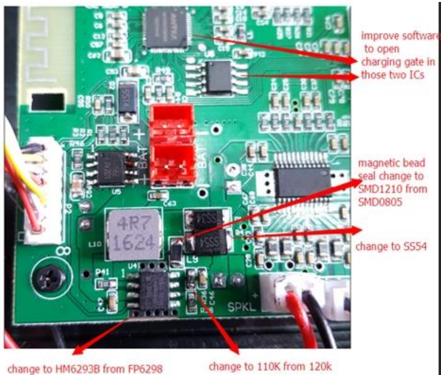
Improved PCBA
