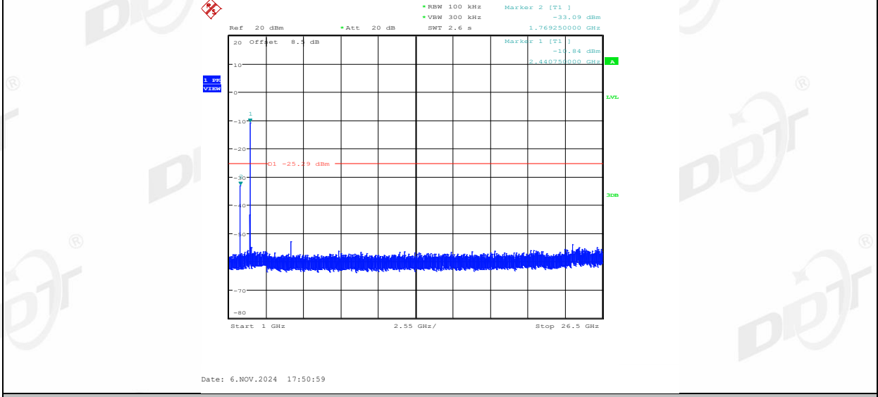
2DH5_Ant2_2480_0~Reference
