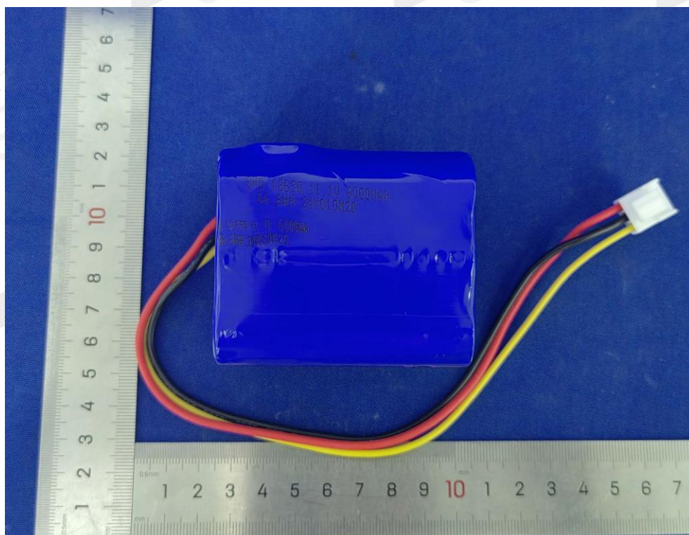
(Battery model: 18650-11.1V-6000mAh-3S3P)
