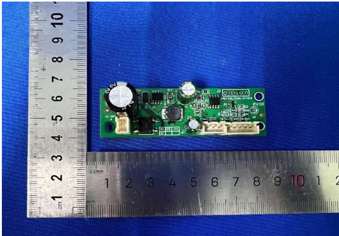
Light control board 1 (Guangzhou brilliant electronic co. LTD)
