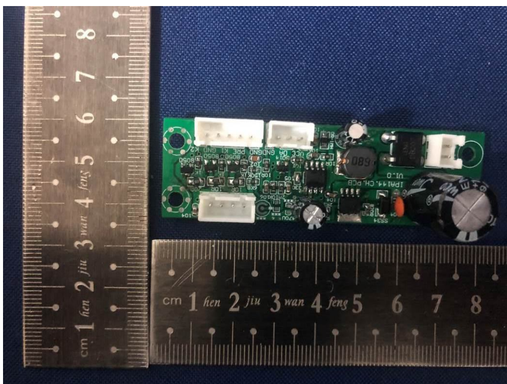
Light control board 2: Guangzhou brilliant electronic co. LTD
