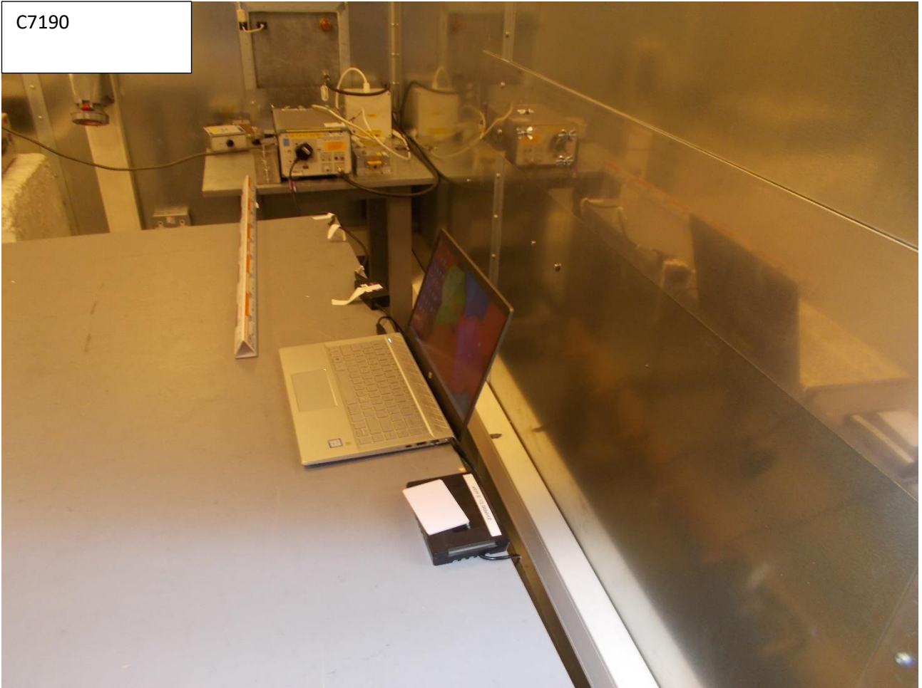
AC Mains Conducted Emissions 150kHz to 30MHz
