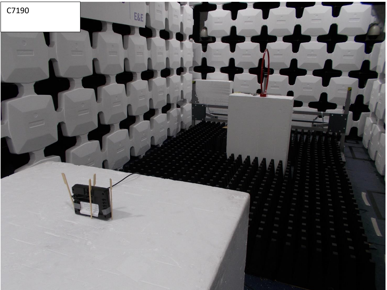
Radiated Magnetic Field Emissions 9kHz to 30MHz
