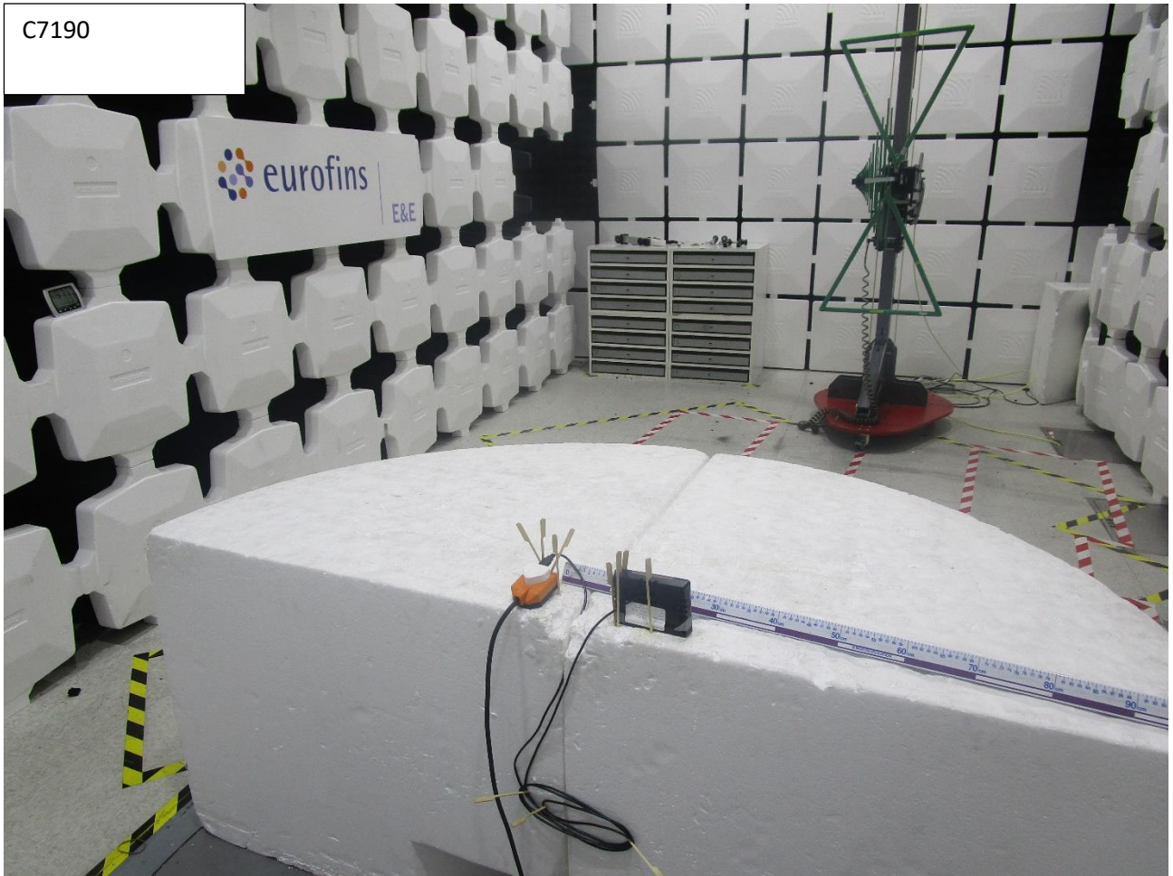
Radiated Electric Field Test 30MHz to1GHz
