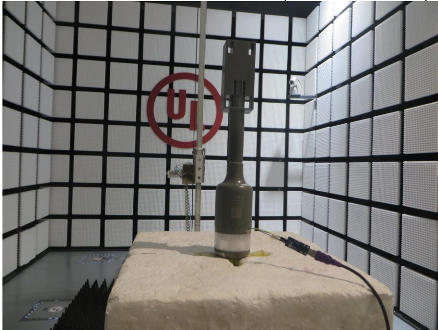
RADIATED RF MEASUREMENT SETUP (ABOVE 1 GHz-Z axis)
