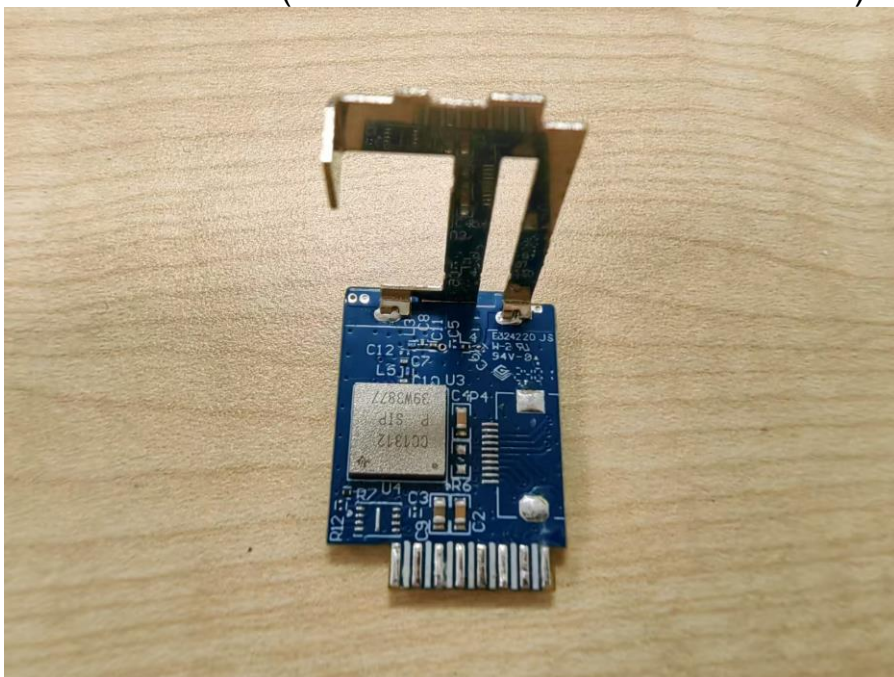
View of EUT-4(condition 2/HVIN: P-SP-A5-01B-A)
