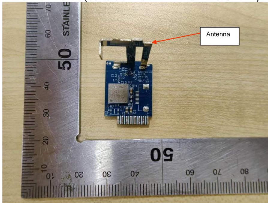
View of EUT-3(condition 2/HVIN: P-SP-A5-01B-A)
