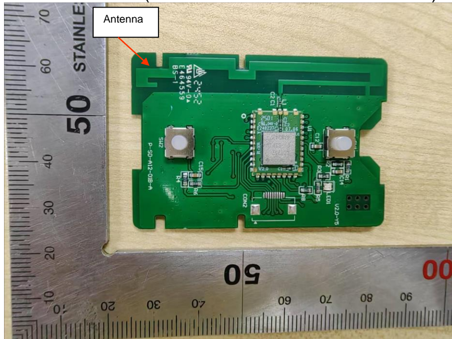
View of EUT-7(condition 4/HVIN: P-SD-A12-01-A)
