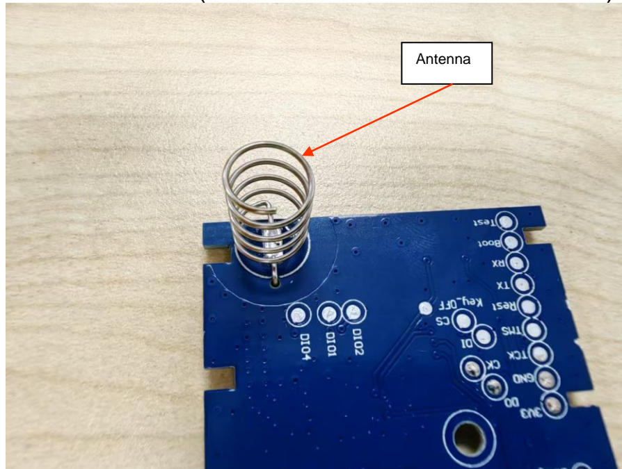
View of EUT-11(condition 5/HVIN: P-SWC-A5-01-A)
