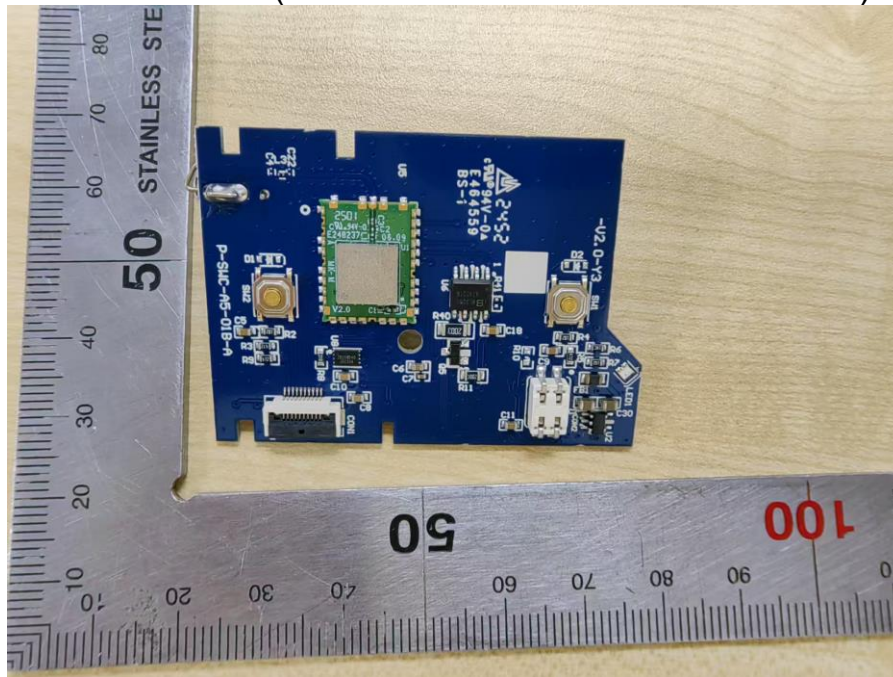
View of EUT-9(condition 5/HVIN: P-SWC-A5-01-A)
