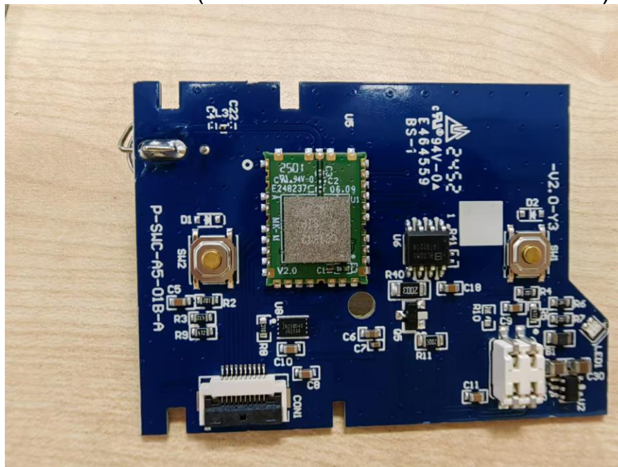
View of EUT-10(condition 5/HVIN: P-SWC-A5-01-A)
