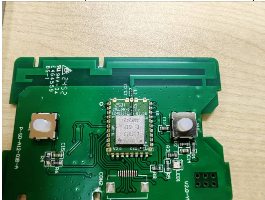
View of EUT-8(condition 4/HVIN: P-SD-A12-01-A)
