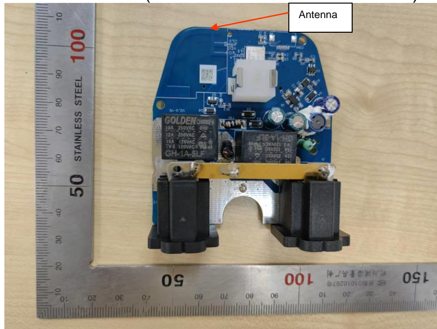
View of EUT-1(condition 1/HVIN: P-SP-A6-01-A)
