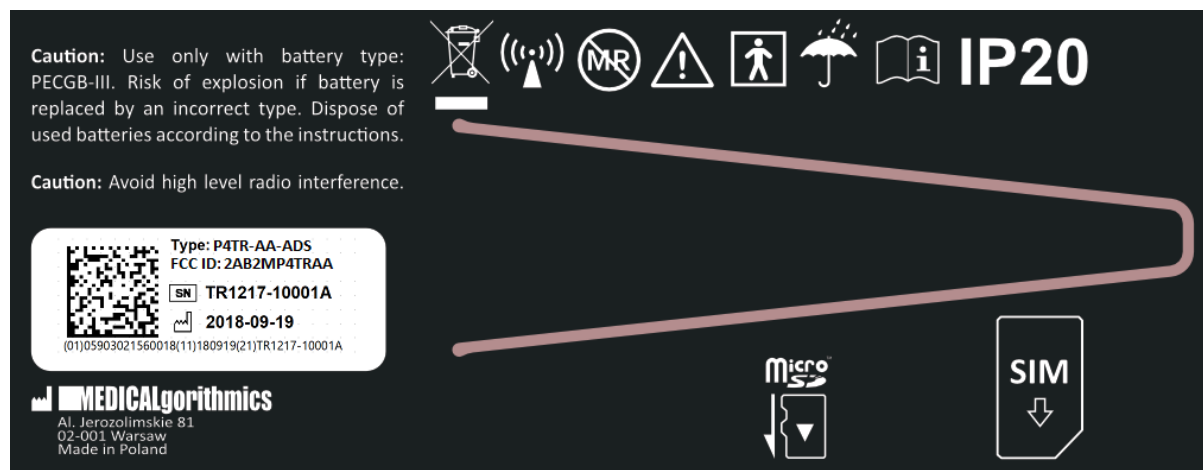
Label for PocketECG transmitter (type P4TR-AA-ADS)
