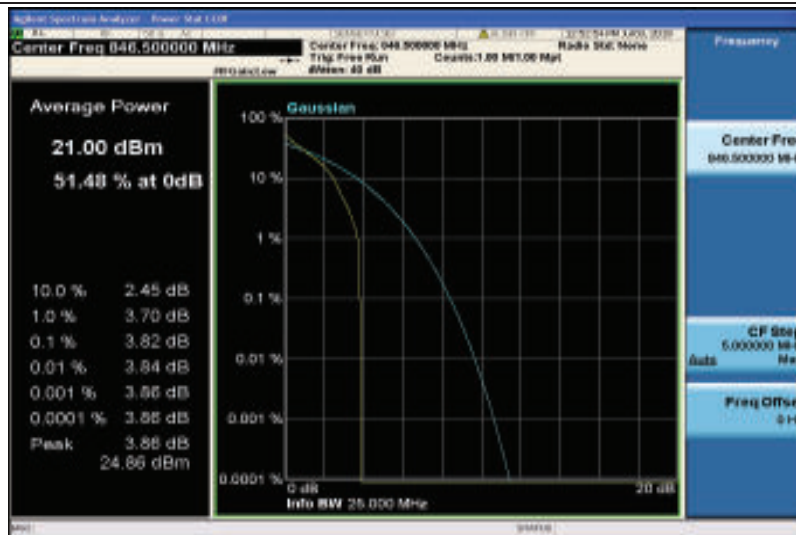
Band26-3MHz-QPSK-27015-15RB#0
