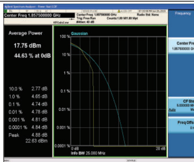
Band25_15MHz_16QAM_26115_1RB#0
