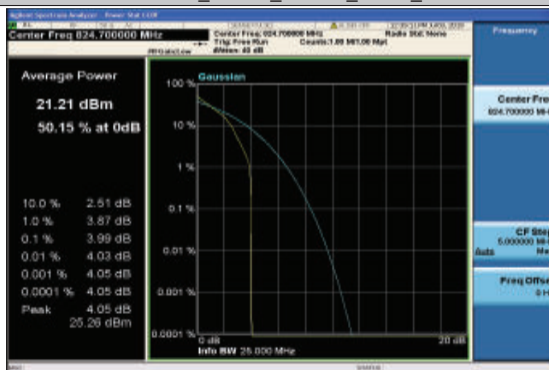
Band26-1.4MHz-QPSK-26797-6RB#0
