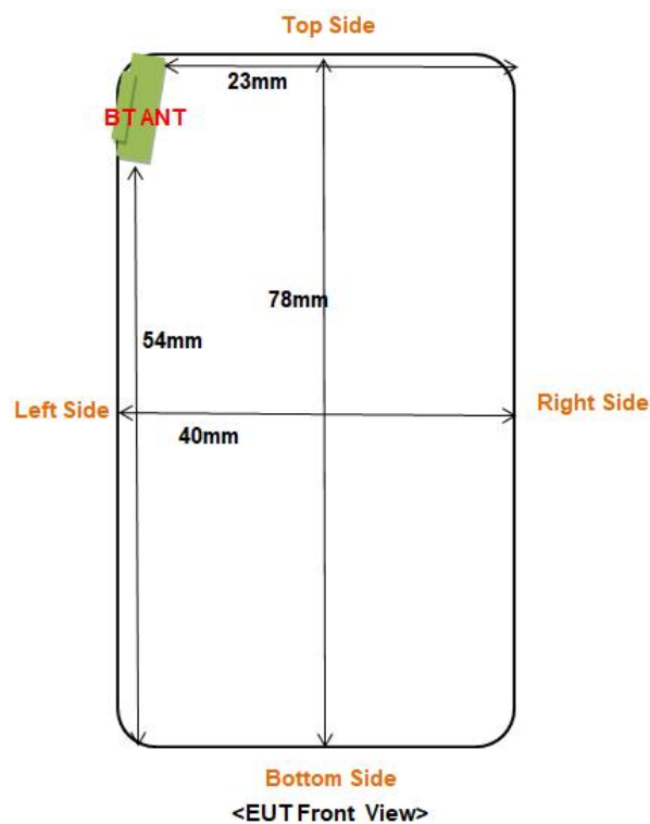
Fig 7.2 Block Diagram for EUT Antenna Position
