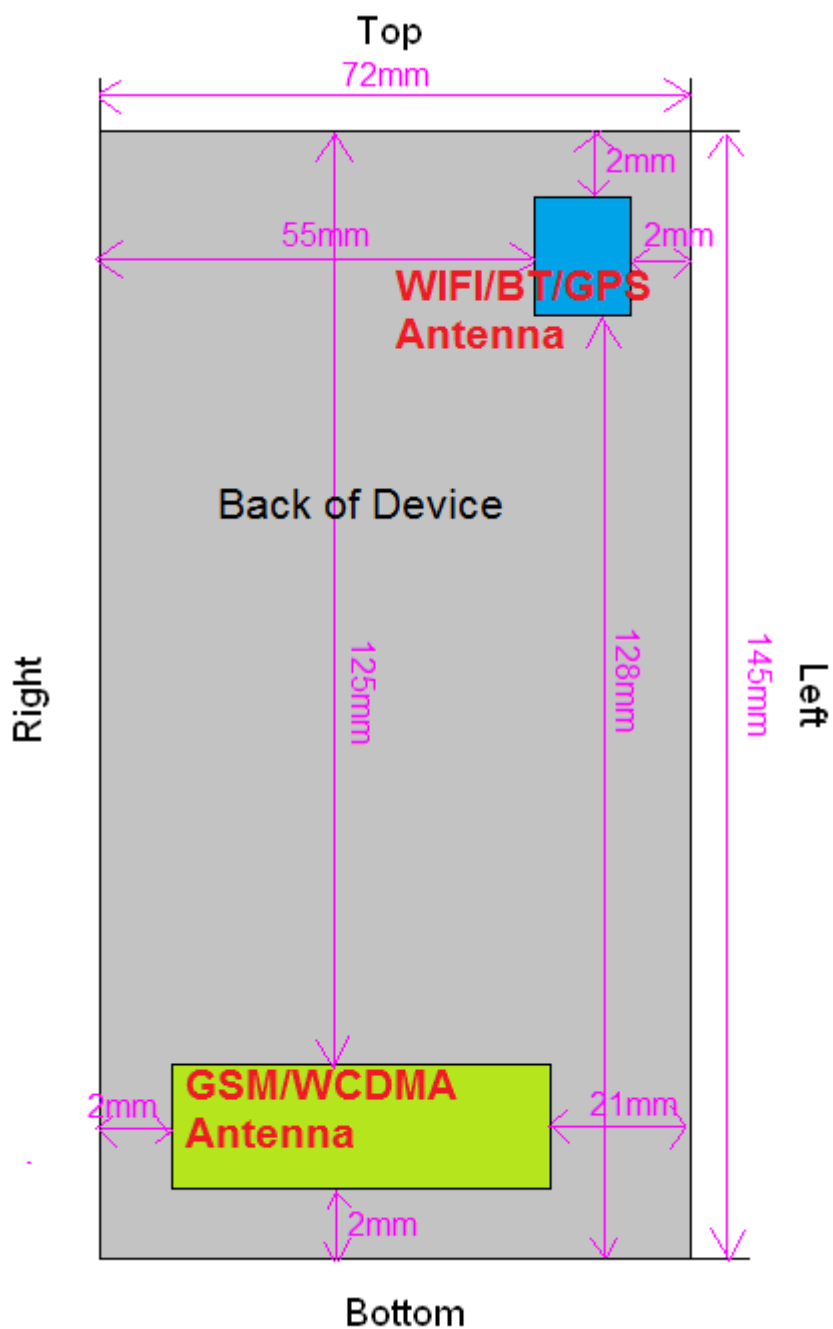
Mobile Test Positions for SAR Testing
