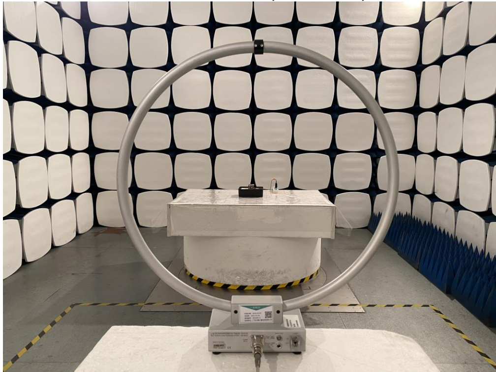
Radiated Emission(9kHz-30MHz)
