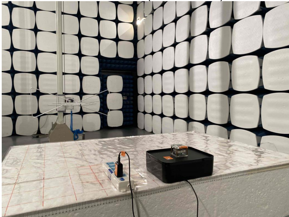
Radiated Emission(30MHz-1000MHz)
