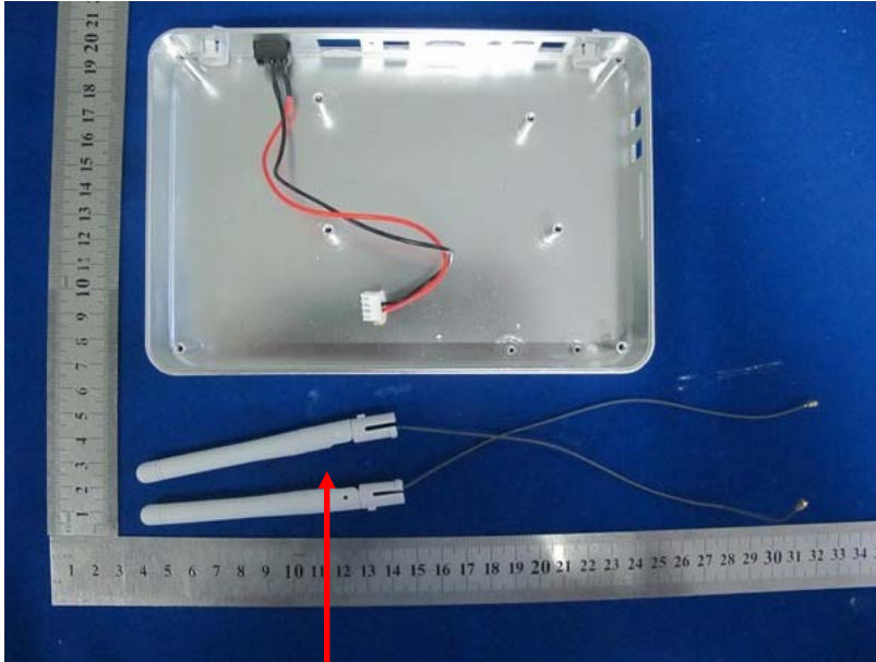
Photo 3 Antennas Photo
