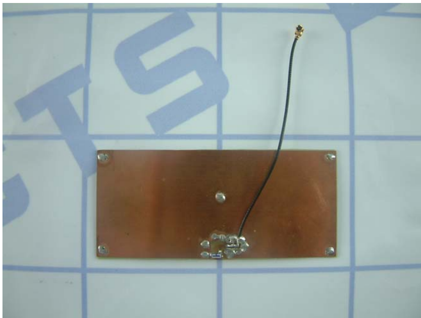
BT Chip Antenna view
