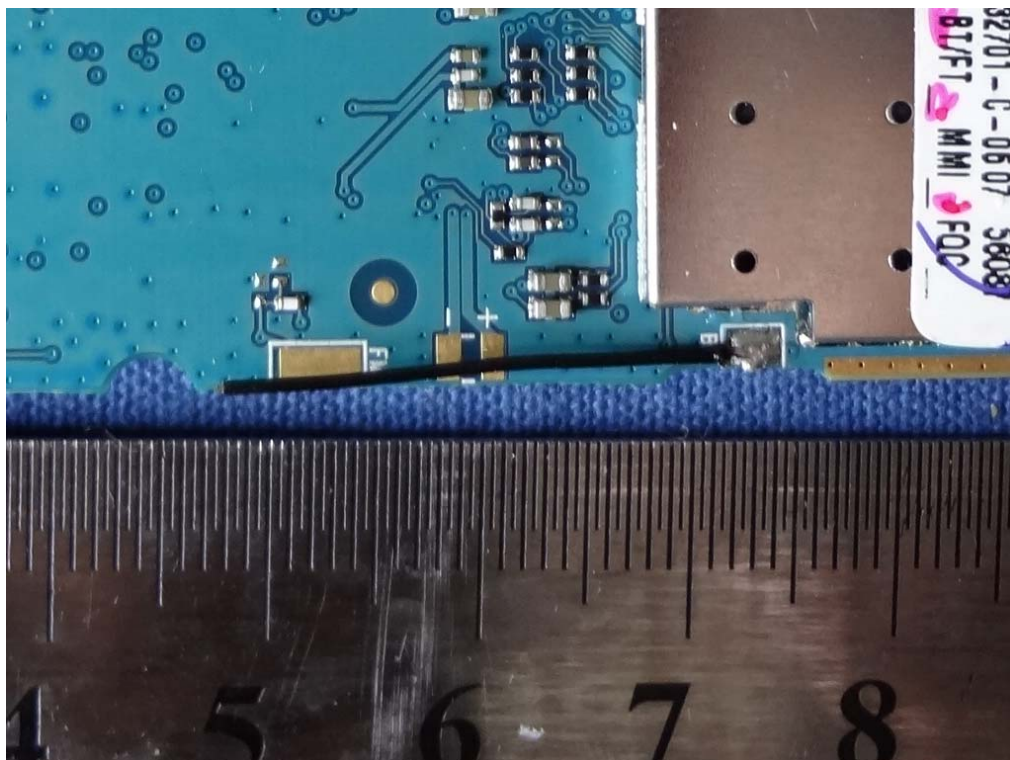
INTERNAL PHOTO OF BT ANTENNA
