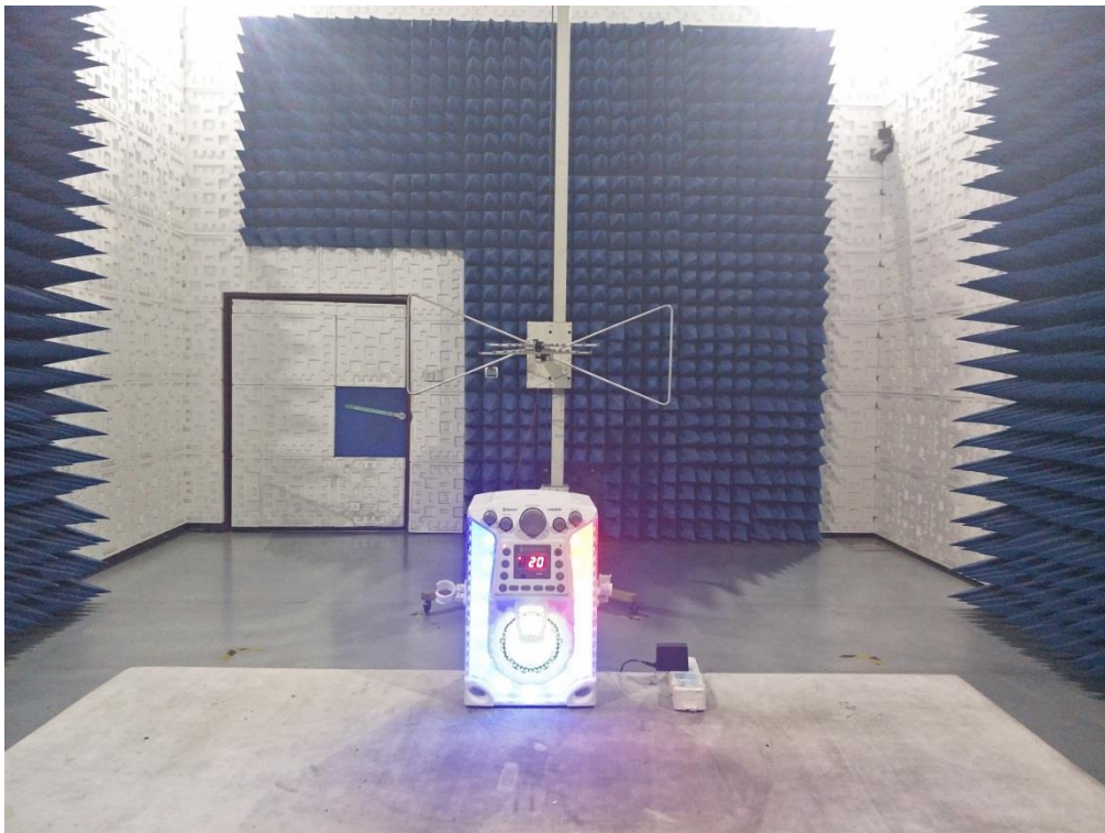
The adapter GKYZA0150058US RADIATED EMISSION TEST SETUP BELOW 1GHz
