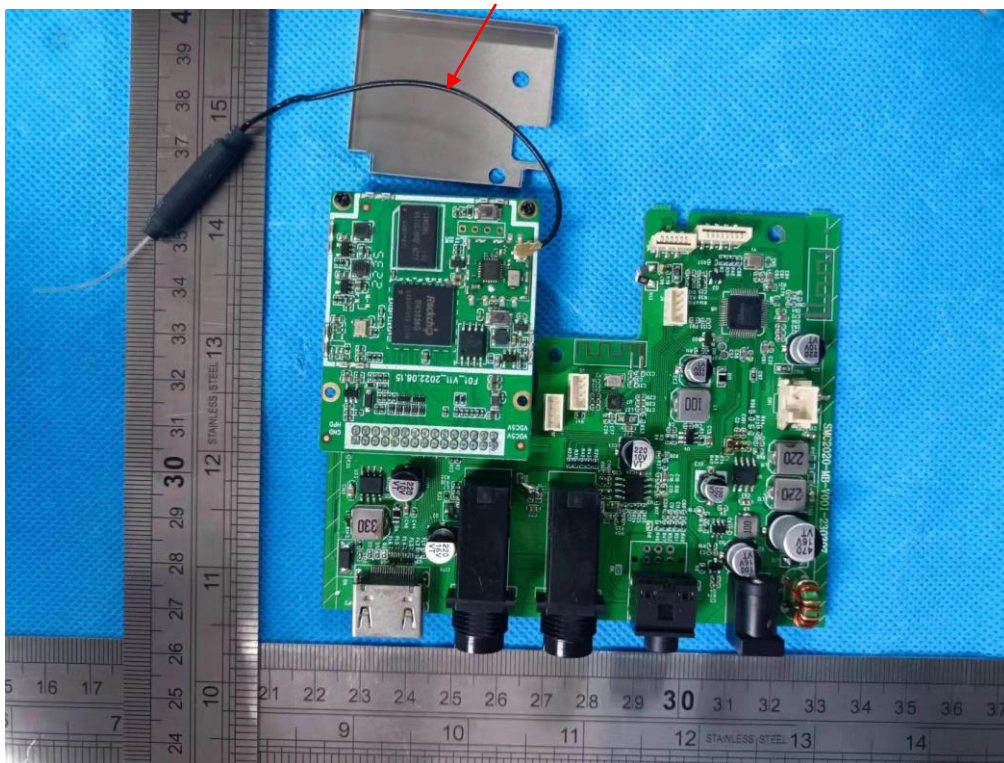
View of wifi antenna
