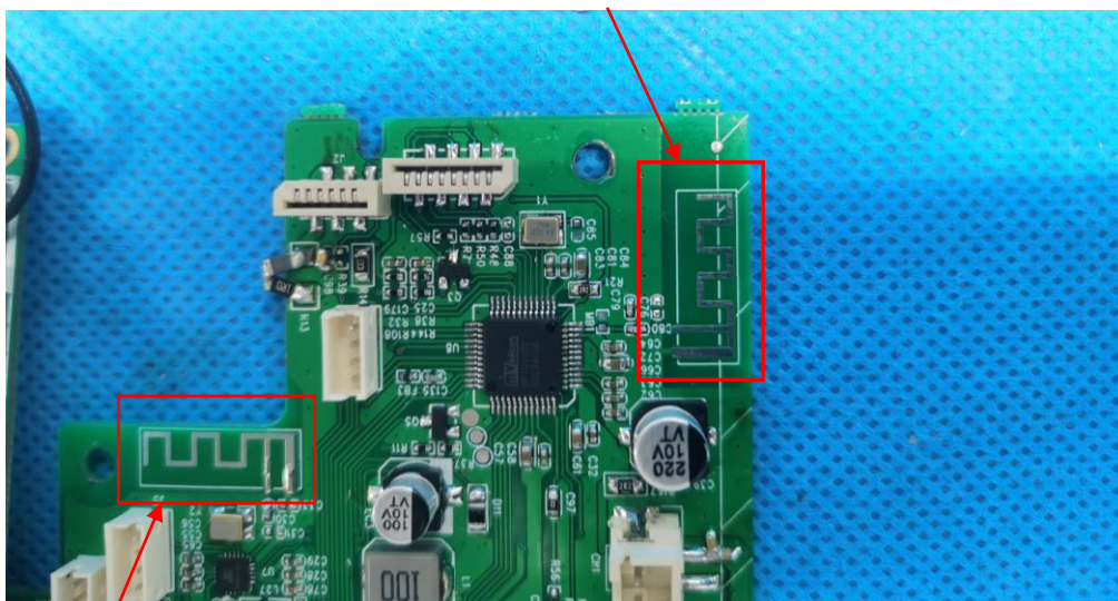
View of BT antenna
