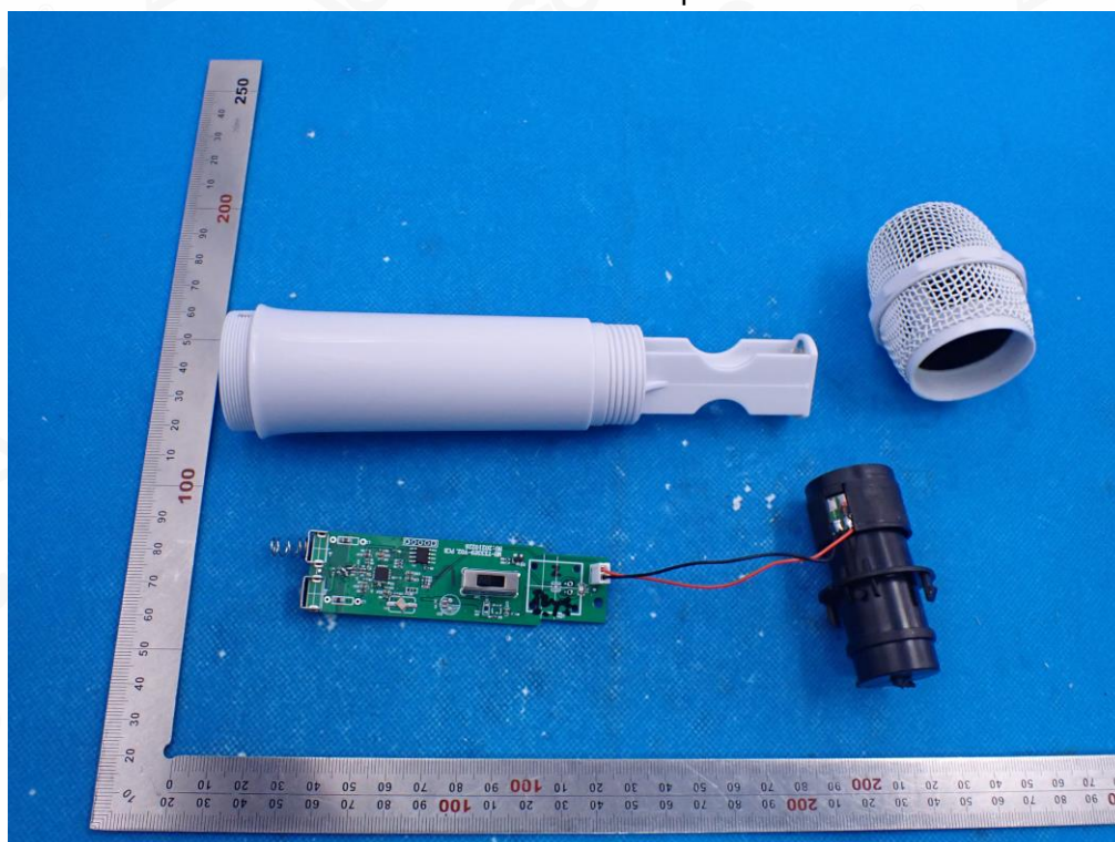
OPEN VIEW OF Microphone
