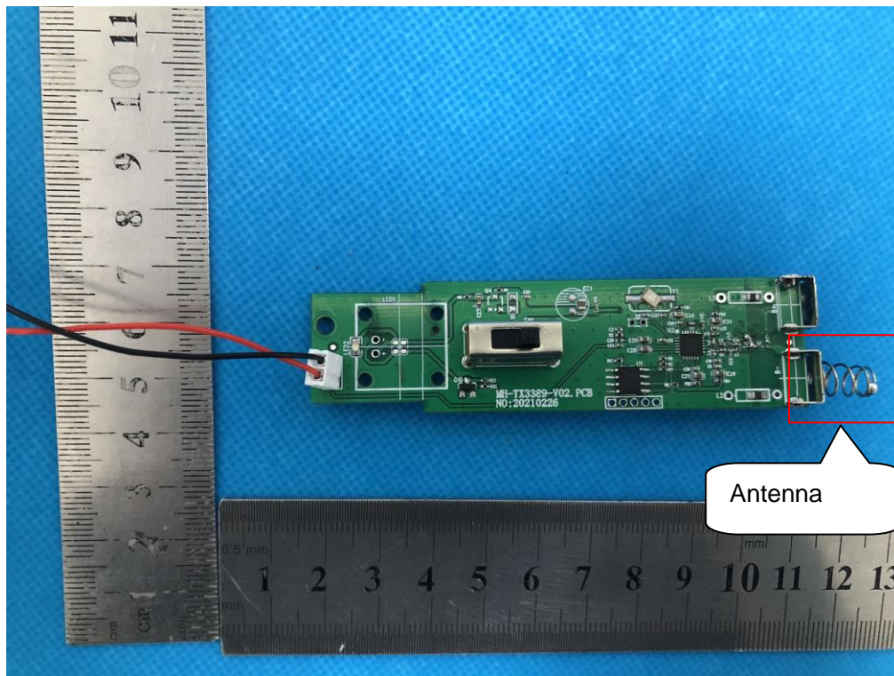
INTERNAL VIEW-1 OF Microphone
