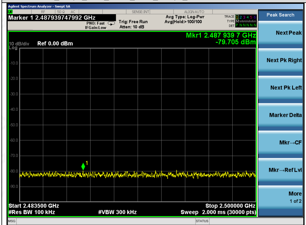
Test Graph EDR ANT1 2480 3Mbps Middle Band Emissions
