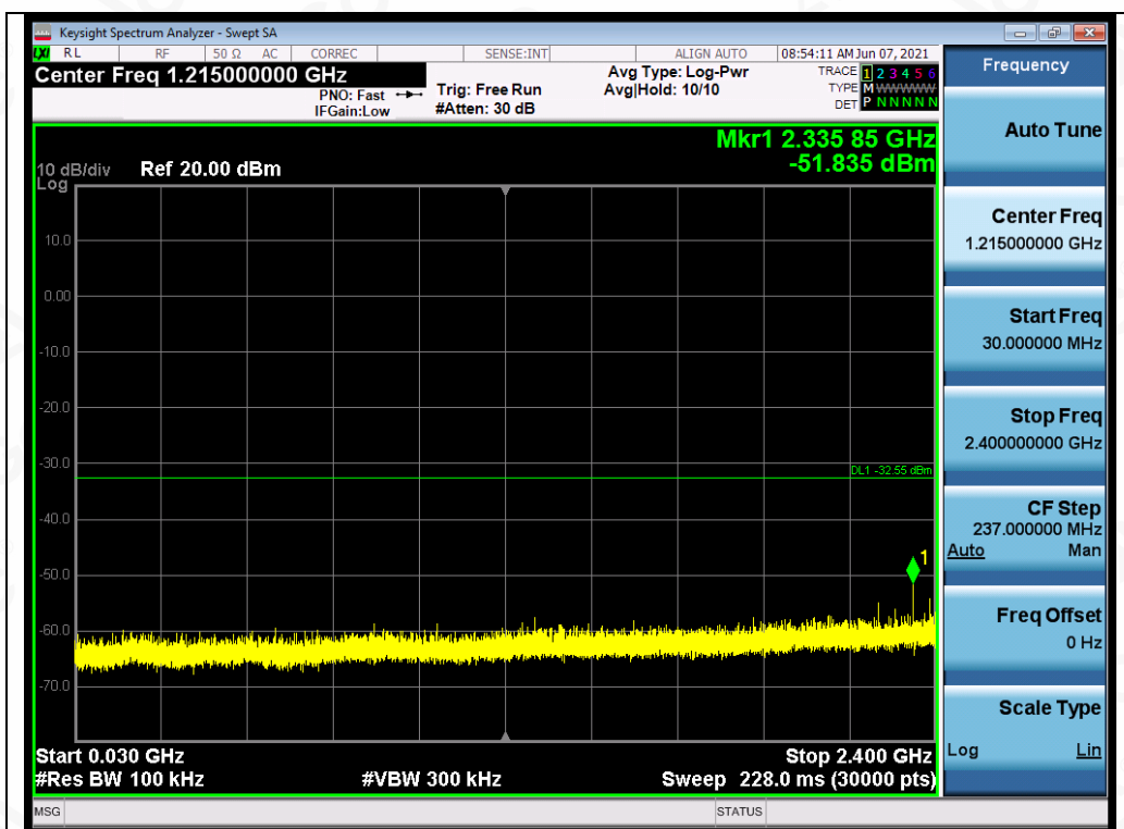
Test Graph EDR ANT1 2480 3Mbps Lower Band Emissions
