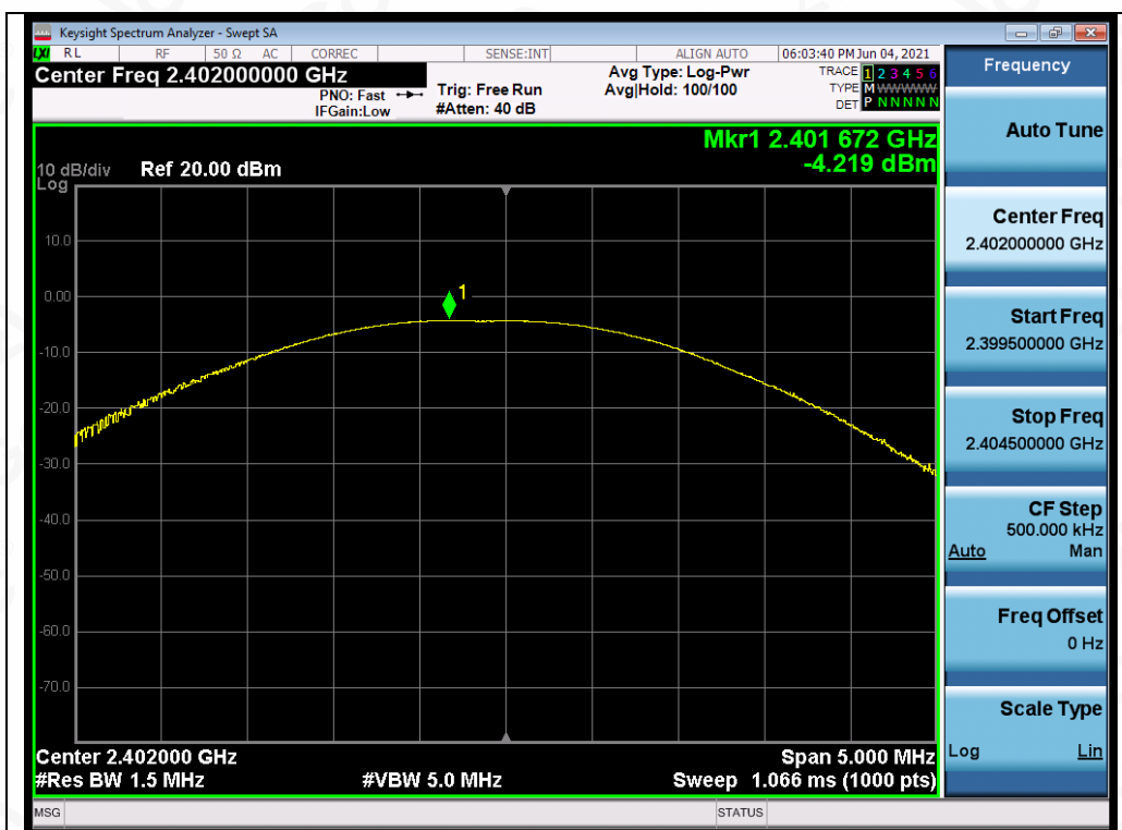
Test Graph EDR ANT1 2402 2Mbps Peak Power
