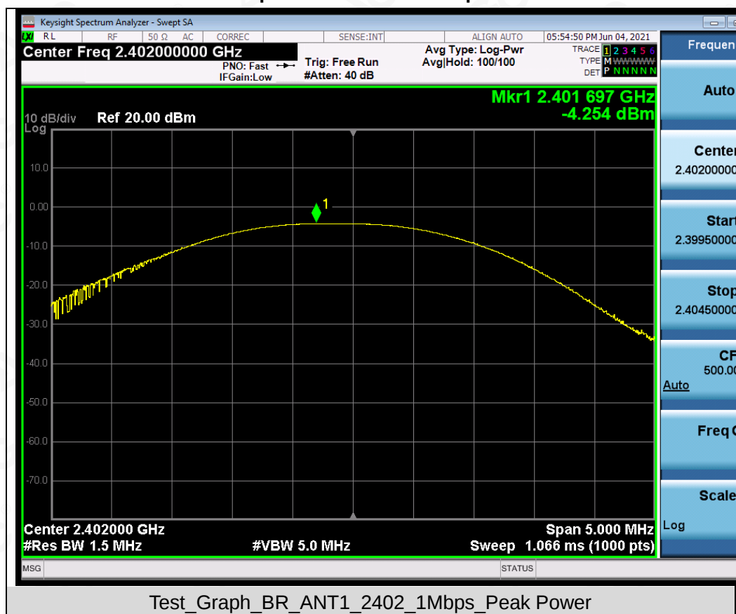
Test Graphs of Conducted Output Power
