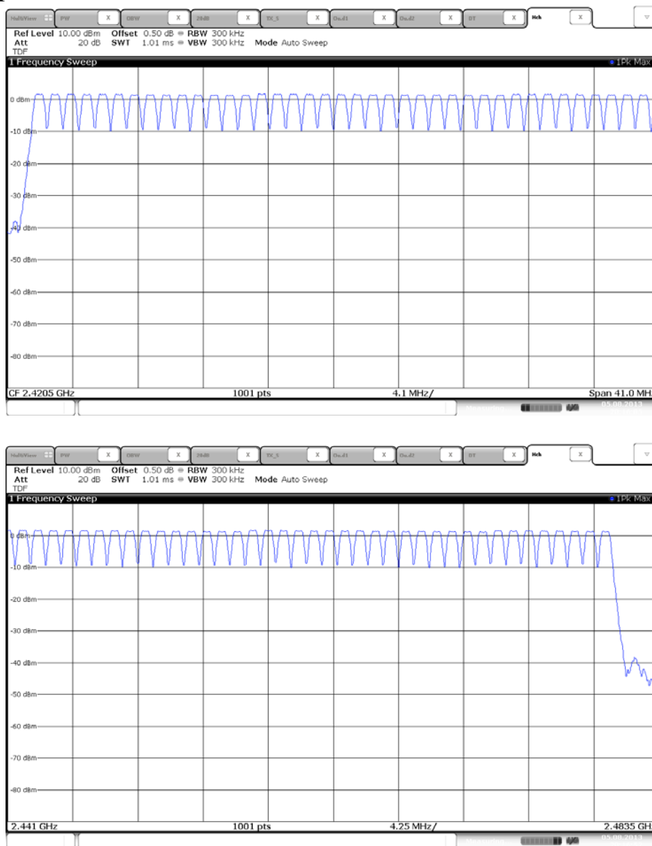
Figure 4. Plot of the Number of Hopping Channels (Conducted)
