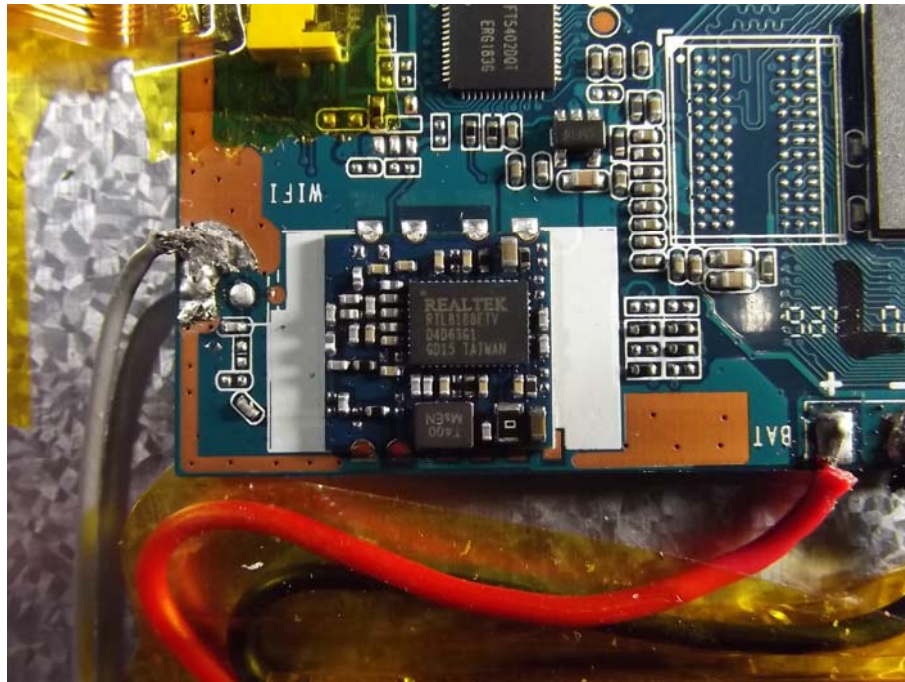
Figure 7 WIFI Module
