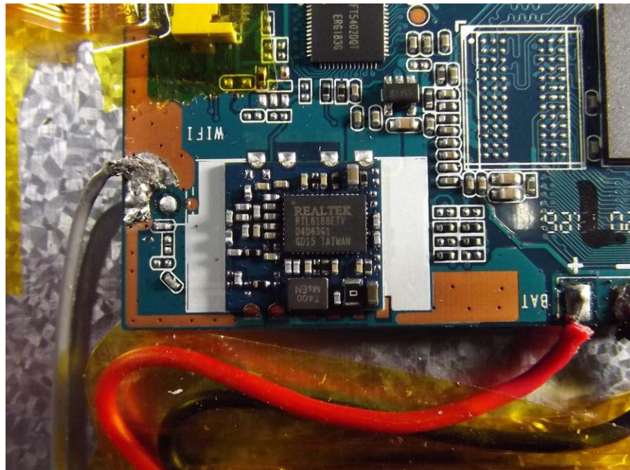
Figure 7 WIFI Module
