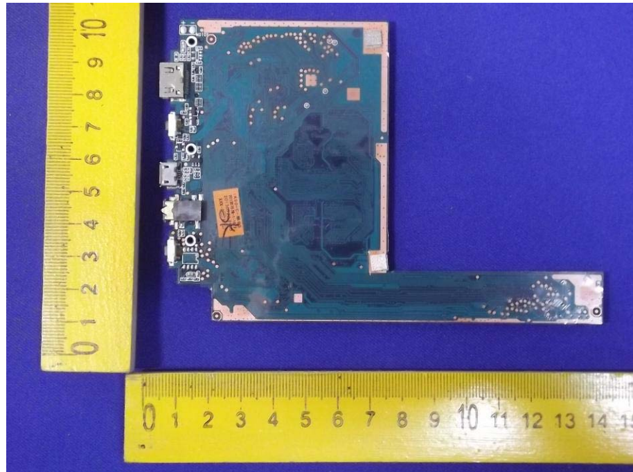
Figure 7 WIFI Module
