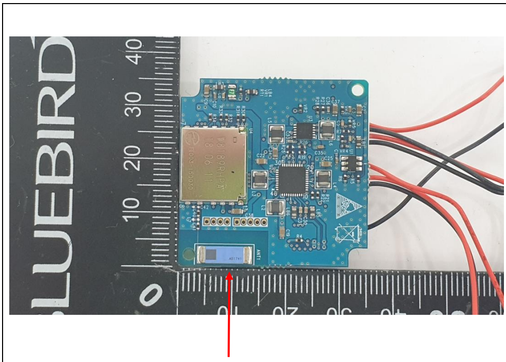
Multilayer Chip Antenna
