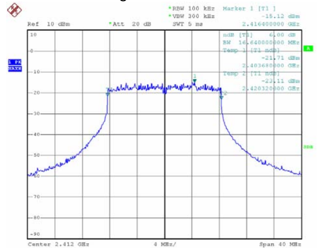
802.11g 2412MHz
