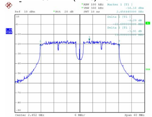
802.11 n (HT40)2452MHz
