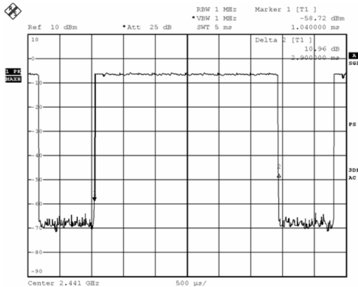
Fig. B [Pulse duration of Middle Channel]
