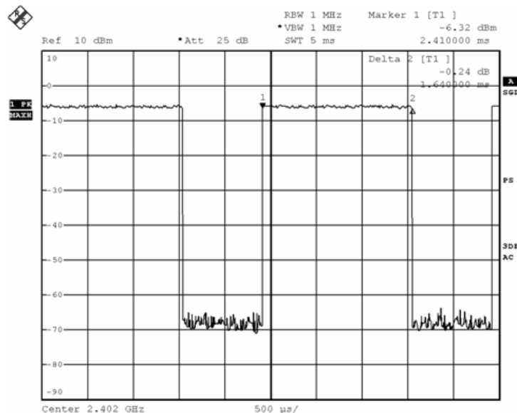
Fig. D [Pulse duration of Lowest Channel]
