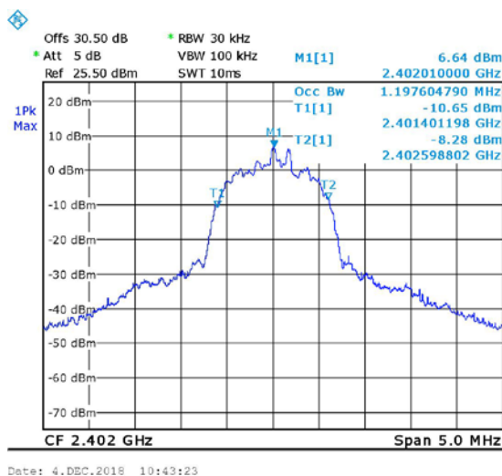
Figure 32. 2402MHz, EDR
