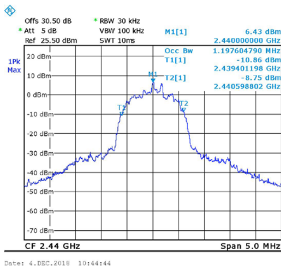
Figure 33. 2440MHz, EDR
