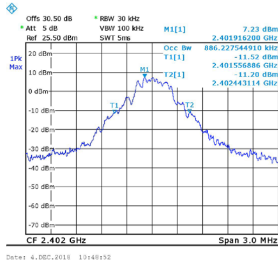
Figure 29. 2402MHz, STD
