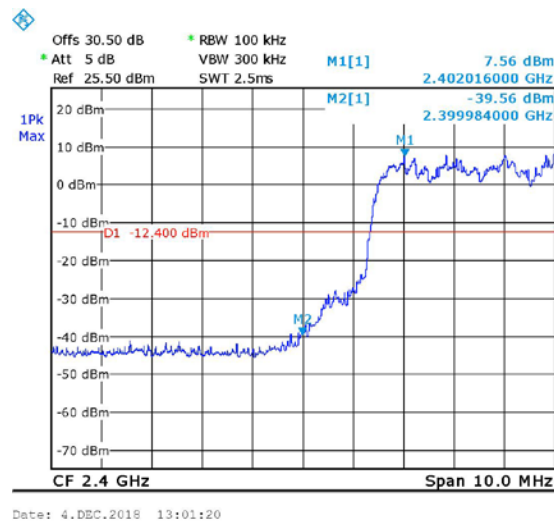
Figure 68 Hopping, Band Edge Low, EDR
