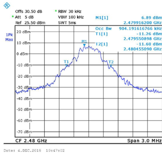
Figure 31. 2480MHz, STD
