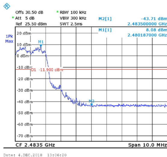
Figure 69 Hopping, Band Edge High, EDR
