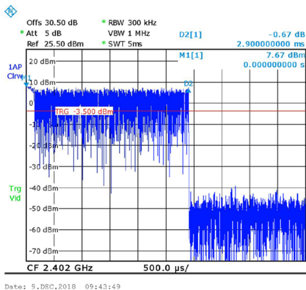
Figure 61 — Burst Duration =2.9msec
