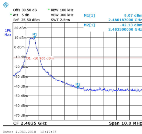
Figure 67 Non-Hopping, Band Edge High, STD
