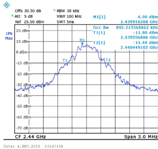
Figure 30. 2440MHz, STD
