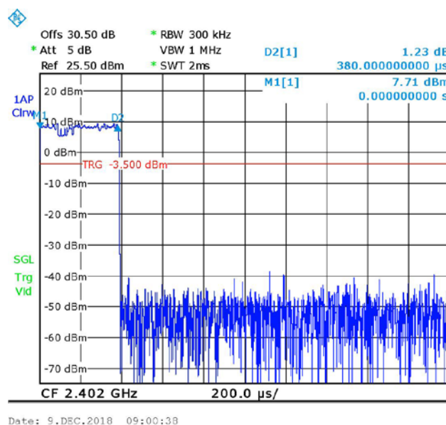
Figure 59 Burst Duration =0.38msec DWELL TIME (31.6 \times 11) \times 0.38m = 132msec < 400msec
