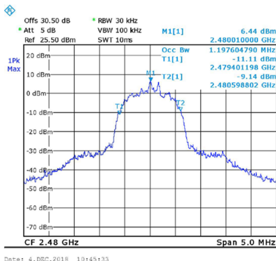
Figure 34. 2480MHz, EDR
