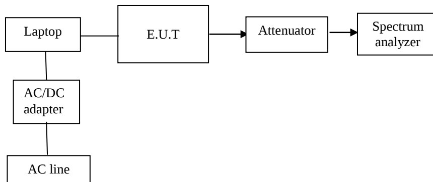
Figure 3. Configuration of Tested System - Conducted
