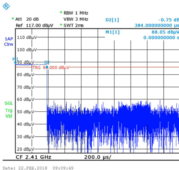
Figure 65 — Burst Duration =0.384msec
