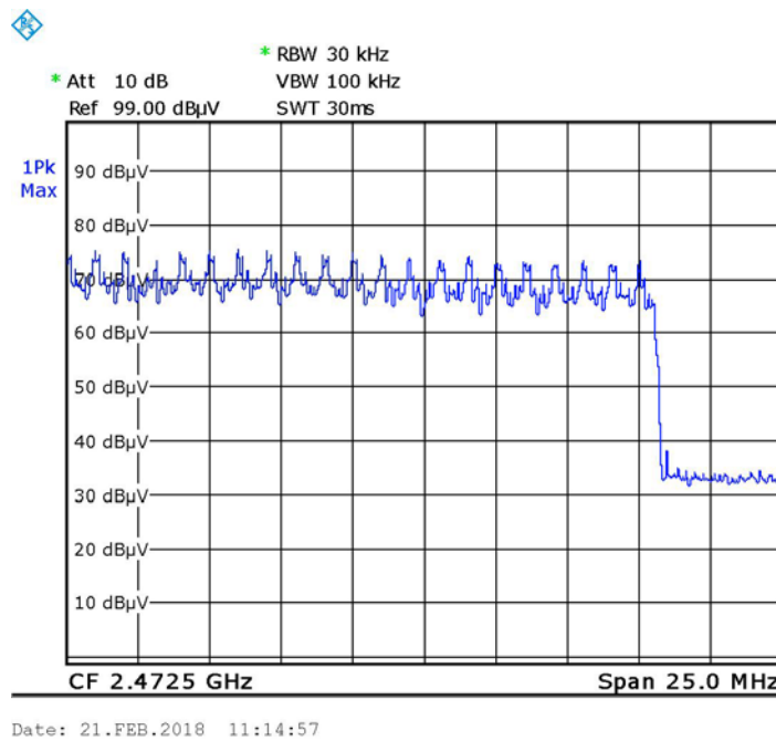
Figure 39. Number of Channels EDR
