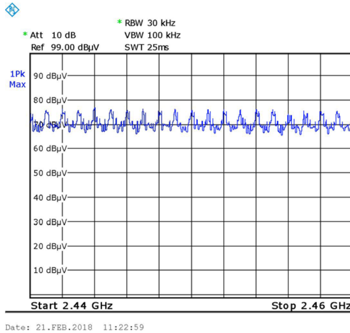
Figure 38. Number of Channels EDR
