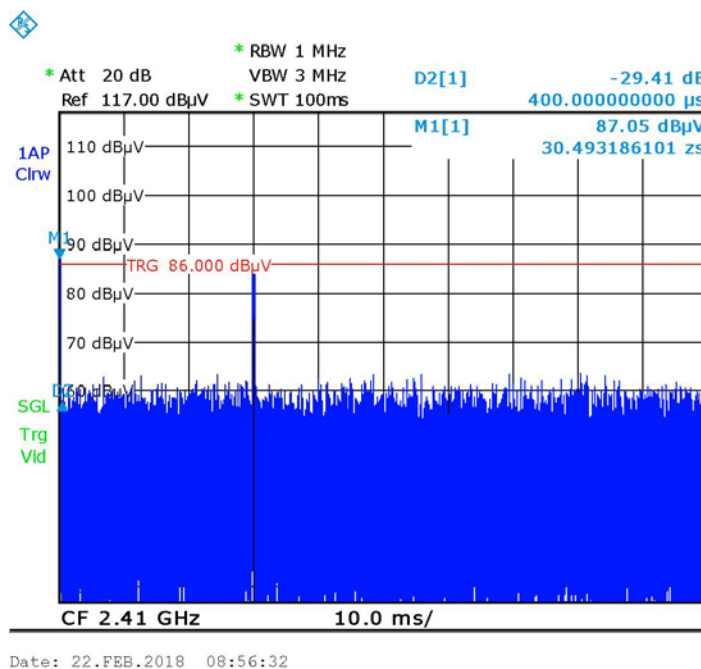
Figure 62 — Number of Bursts in 100msec=2, in 1sec=20
