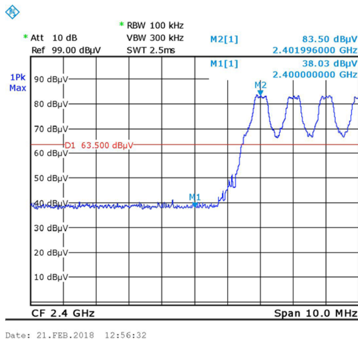
Figure 72 — Hopping – Low, STD.
