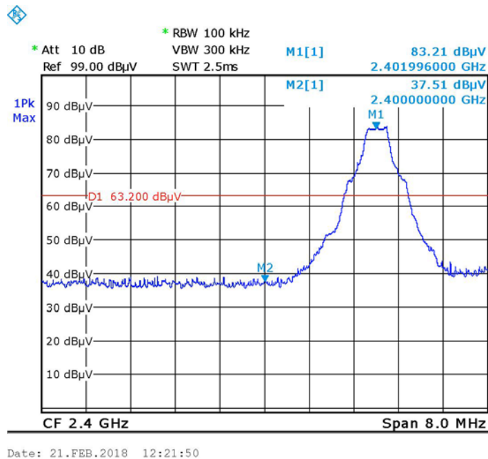
Figure 74 — Non-Hopping – Low, STD.
