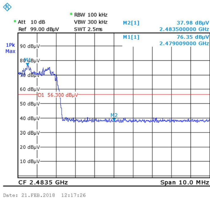
Figure 69 — Hopping – High, EDR
