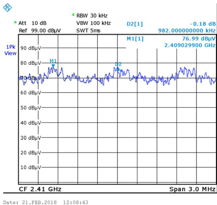
Figure 46. Channel Frequency Separation, EDR
