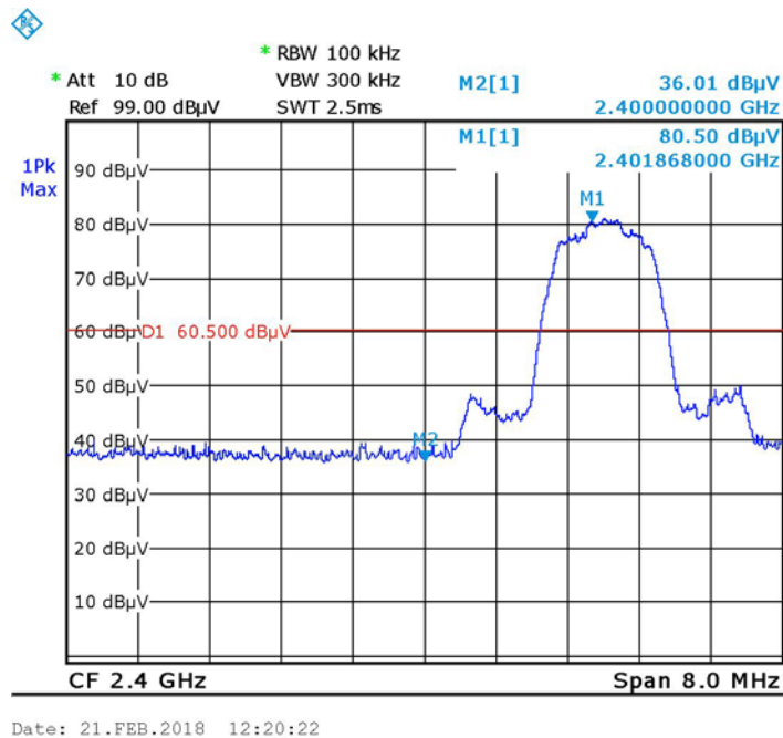
Figure 70 — Non-Hopping – Low, EDR
