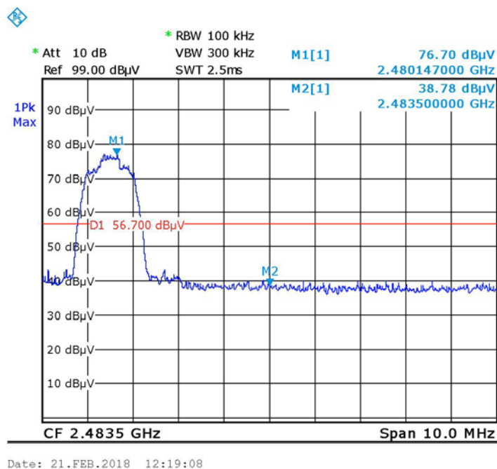
Figure 71 — Non-Hopping – High, EDR
