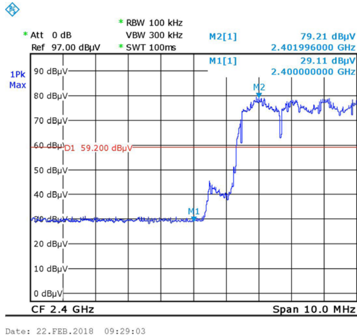
Figure 68 — Hopping – Low, EDR
