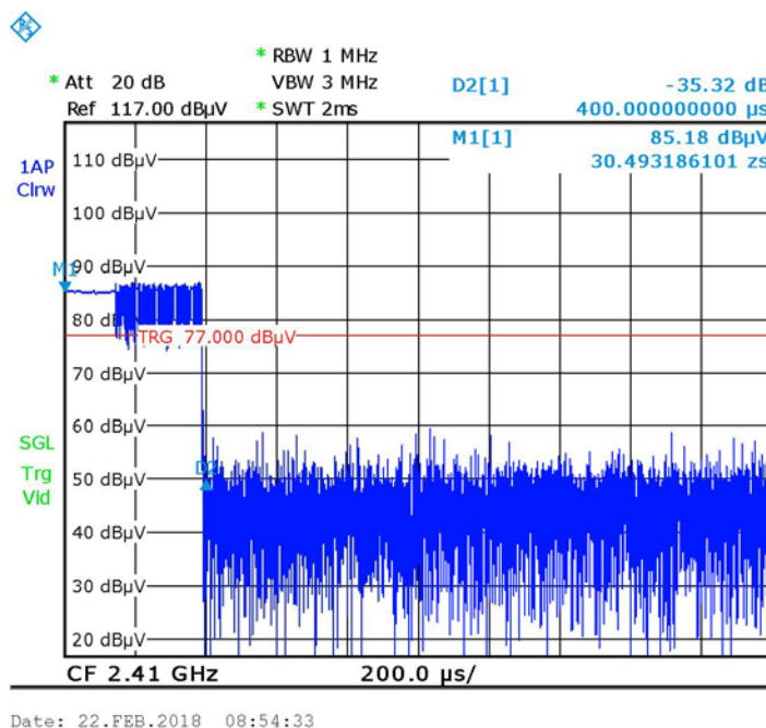
Figure 63 — Burst Duration =0.4msec
