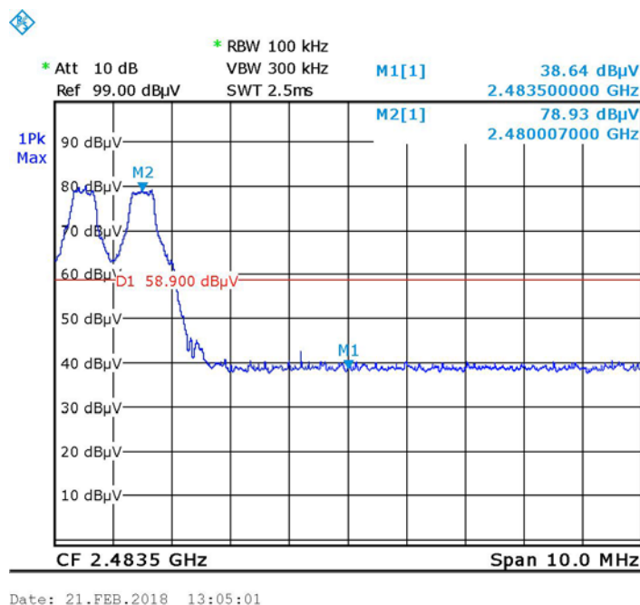
Figure 73 — Hopping – High, STD.
