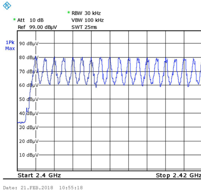
Figure 40. Number of Channels STD.
