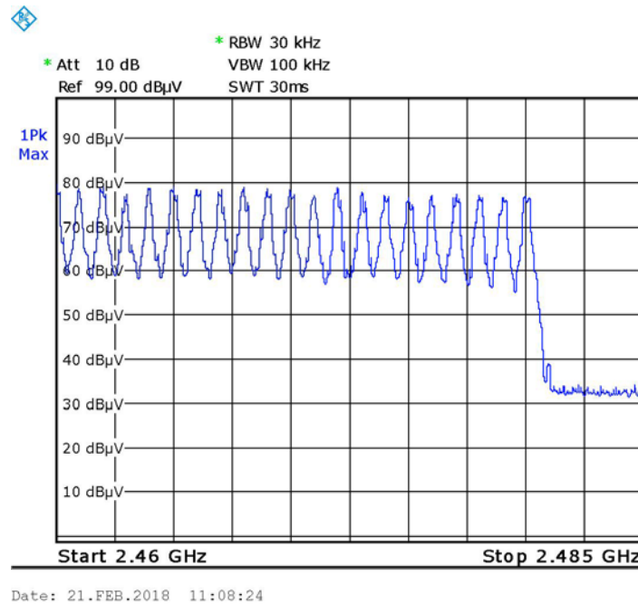
Figure 43. Number of Channels STD.
