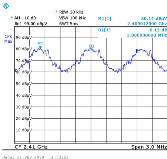
Figure 30. Channel Frequency Separation, STD.
