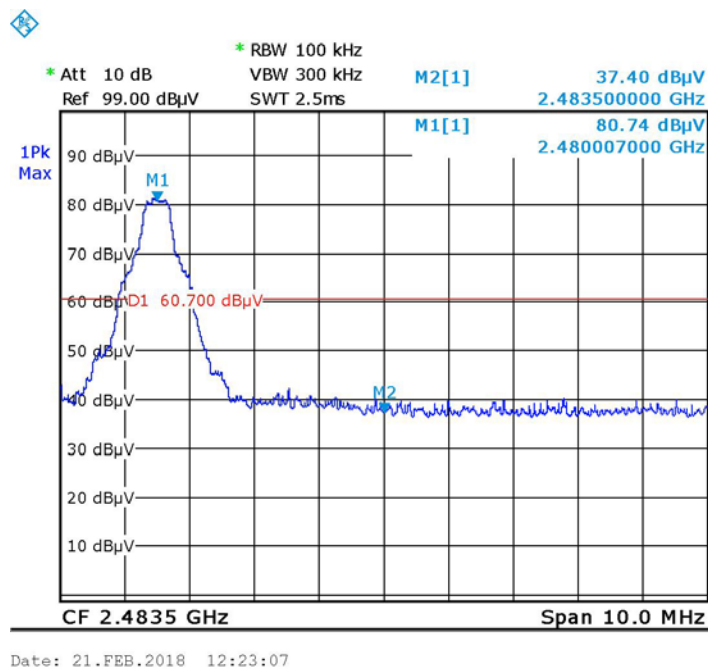
Figure 75 — Non-Hopping – High, STD.
